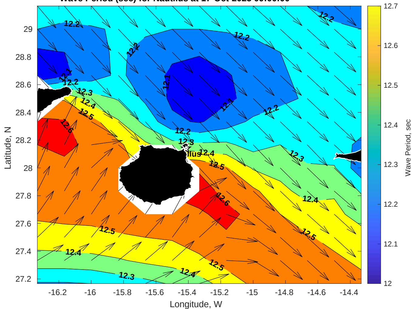
Wave Period (sec) for Nautilus at 17-Oct-2025 09:00:00
