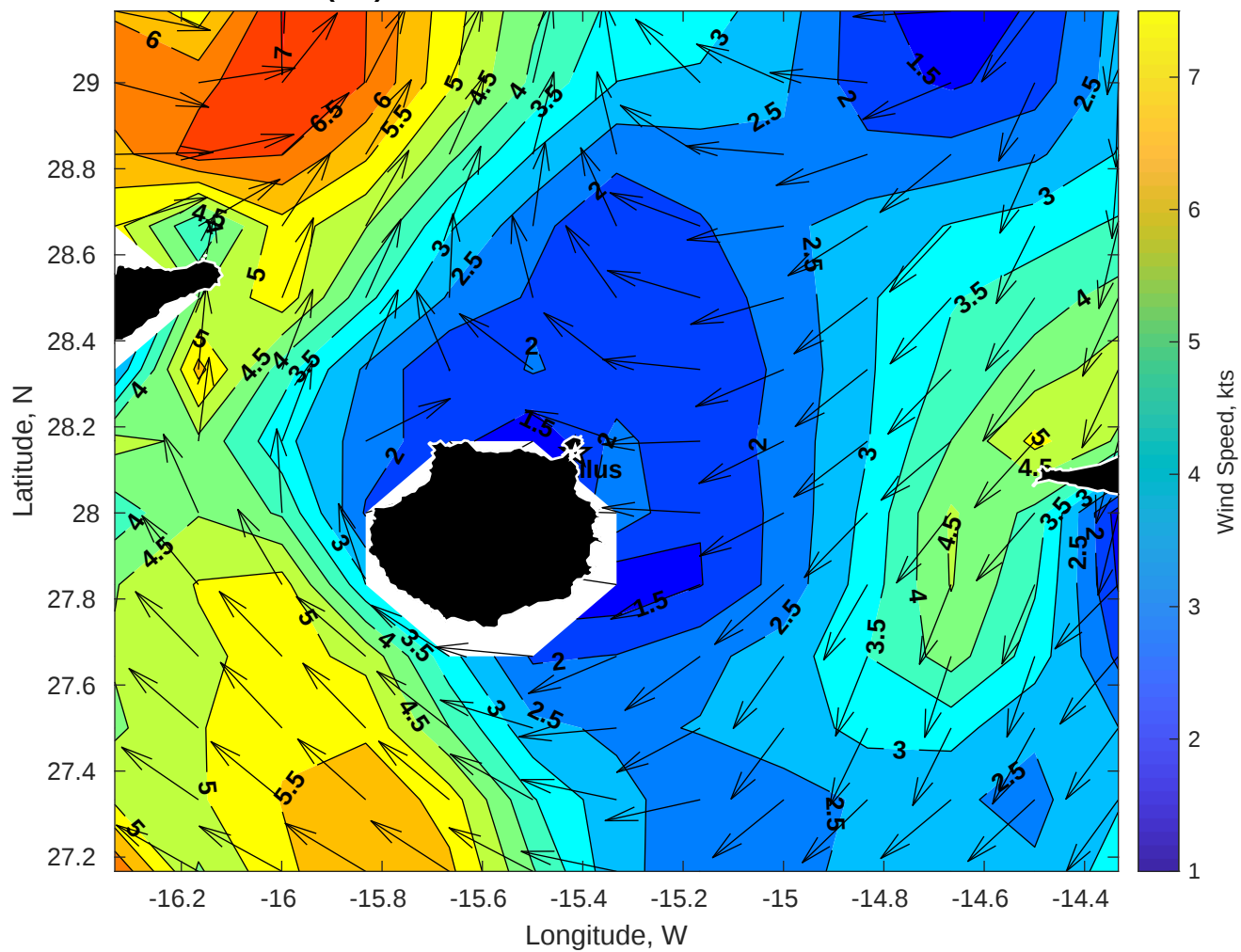
Winds (kts) for Nautilus at 17-Oct-2025 09:00:00
