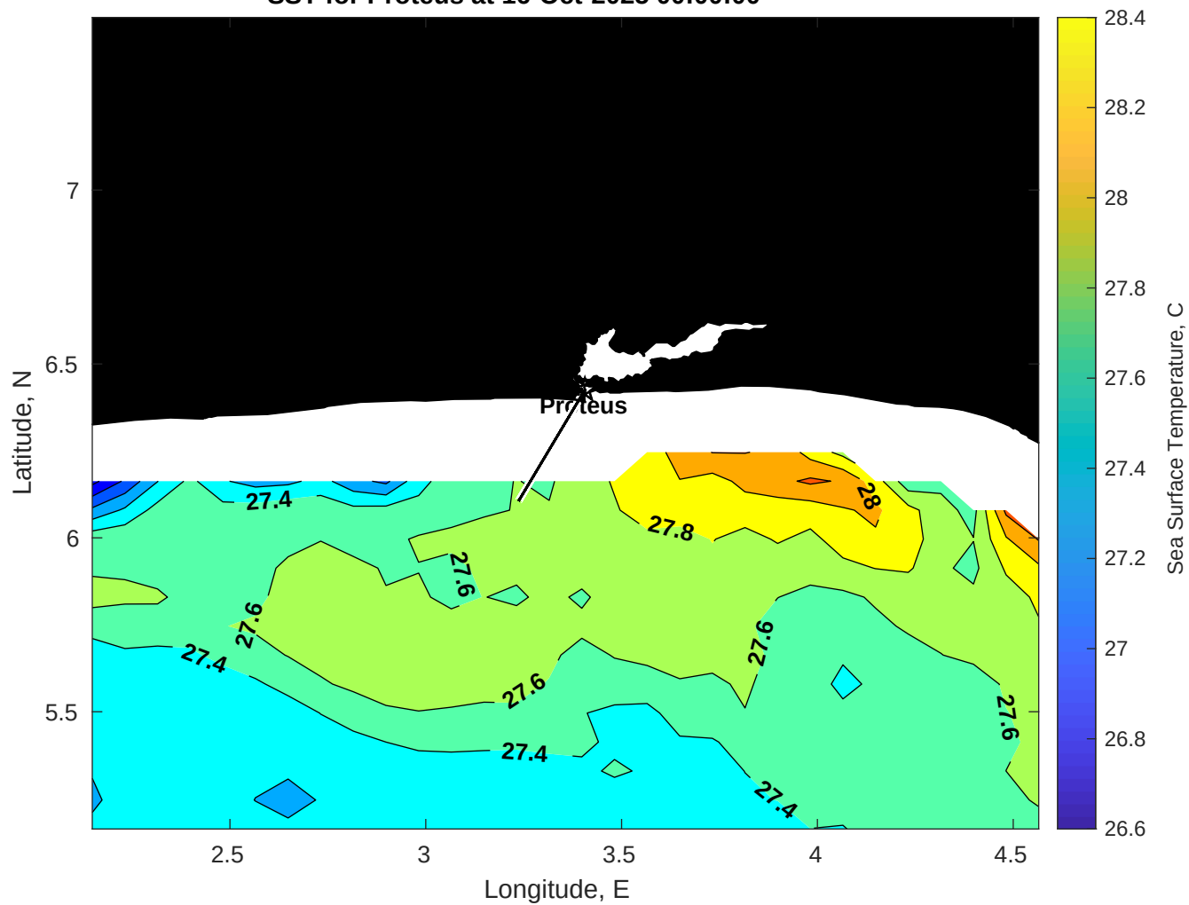
SST for Proteus at 16-Oct-2025 00:00:00
