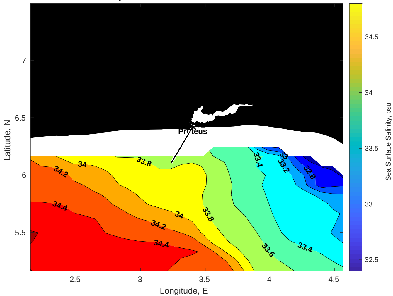
Surface Salinity for Proteus at 16-Oct-2025 00:00:00
