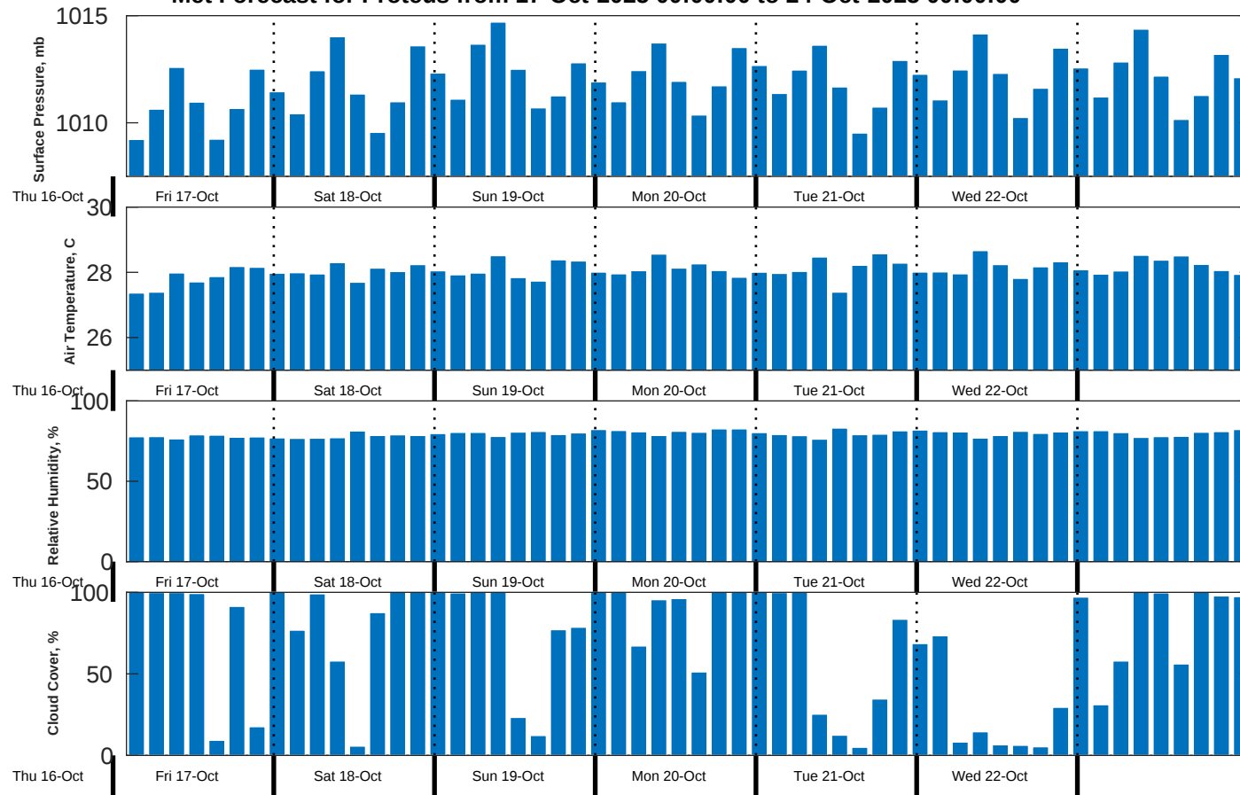
Met Forecast for Proteus from 17-Oct-2025 00:00:00 to 24-Oct-2025 00:00:00
