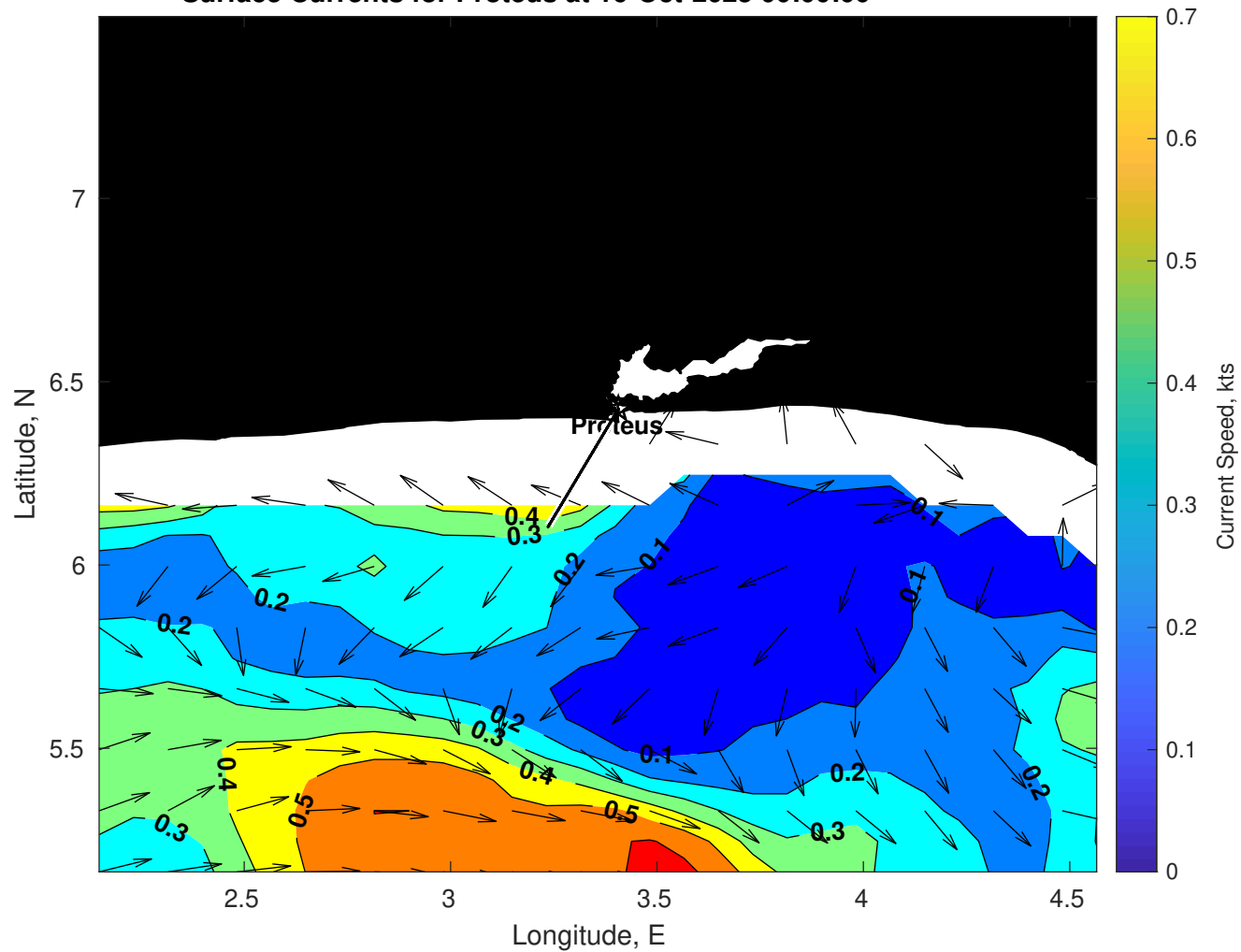
Surface Currents for Proteus at 16-Oct-2025 00:00:00
