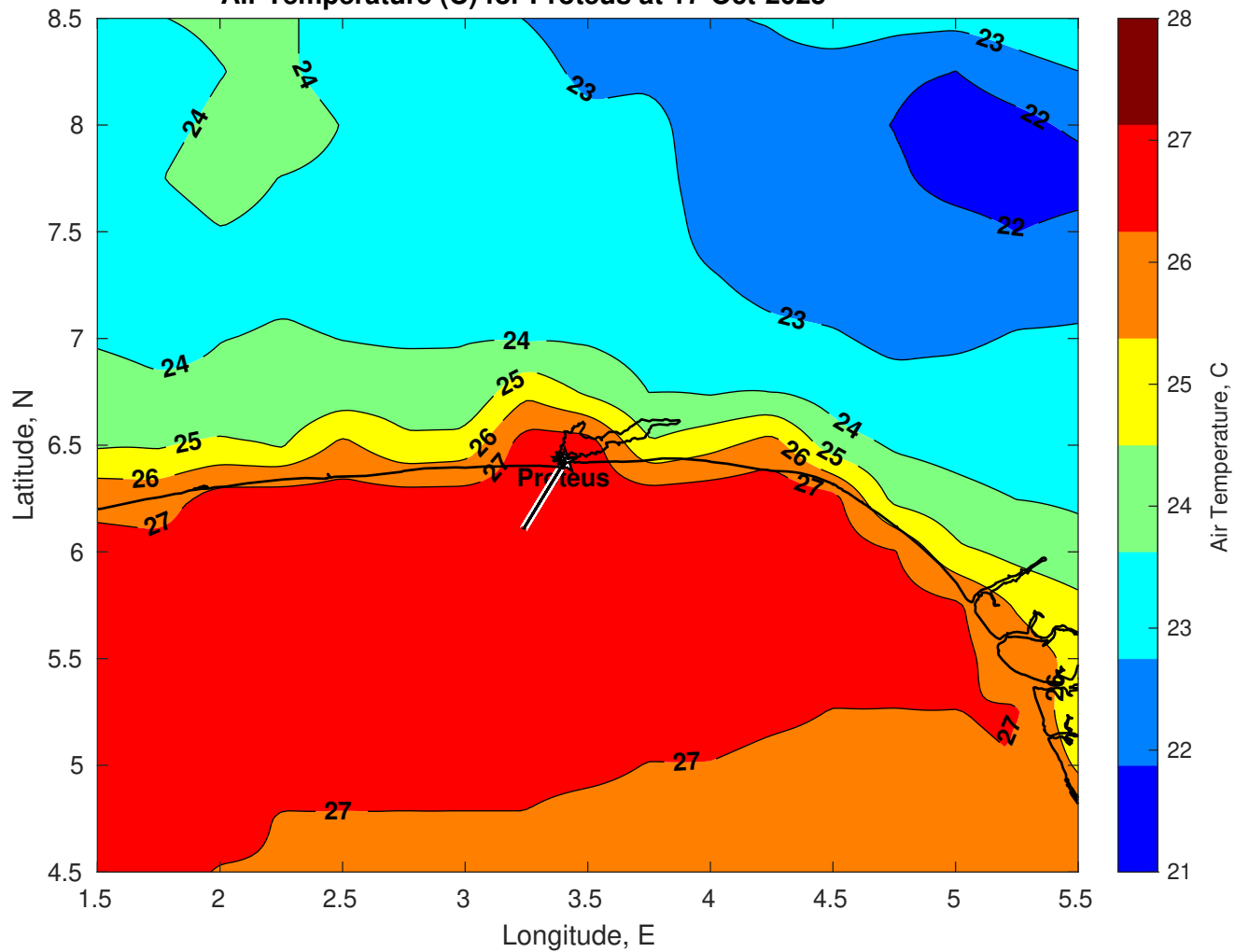
Air Temperature (C) for Proteus at 17-Oct-2025
