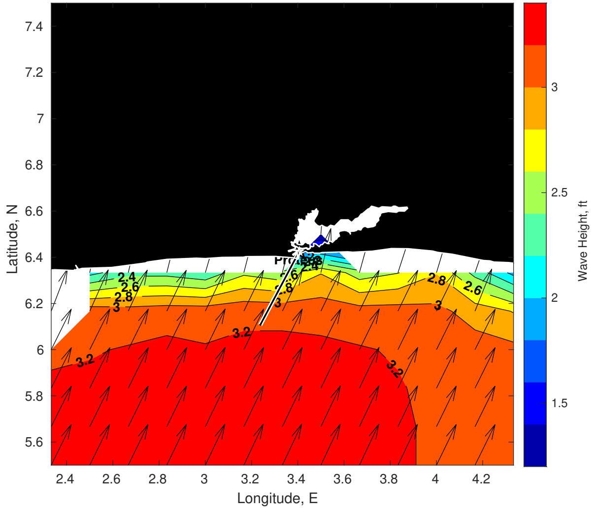
Wave Height (ft) for Proteus at 17-Oct-2025 09:00:00
