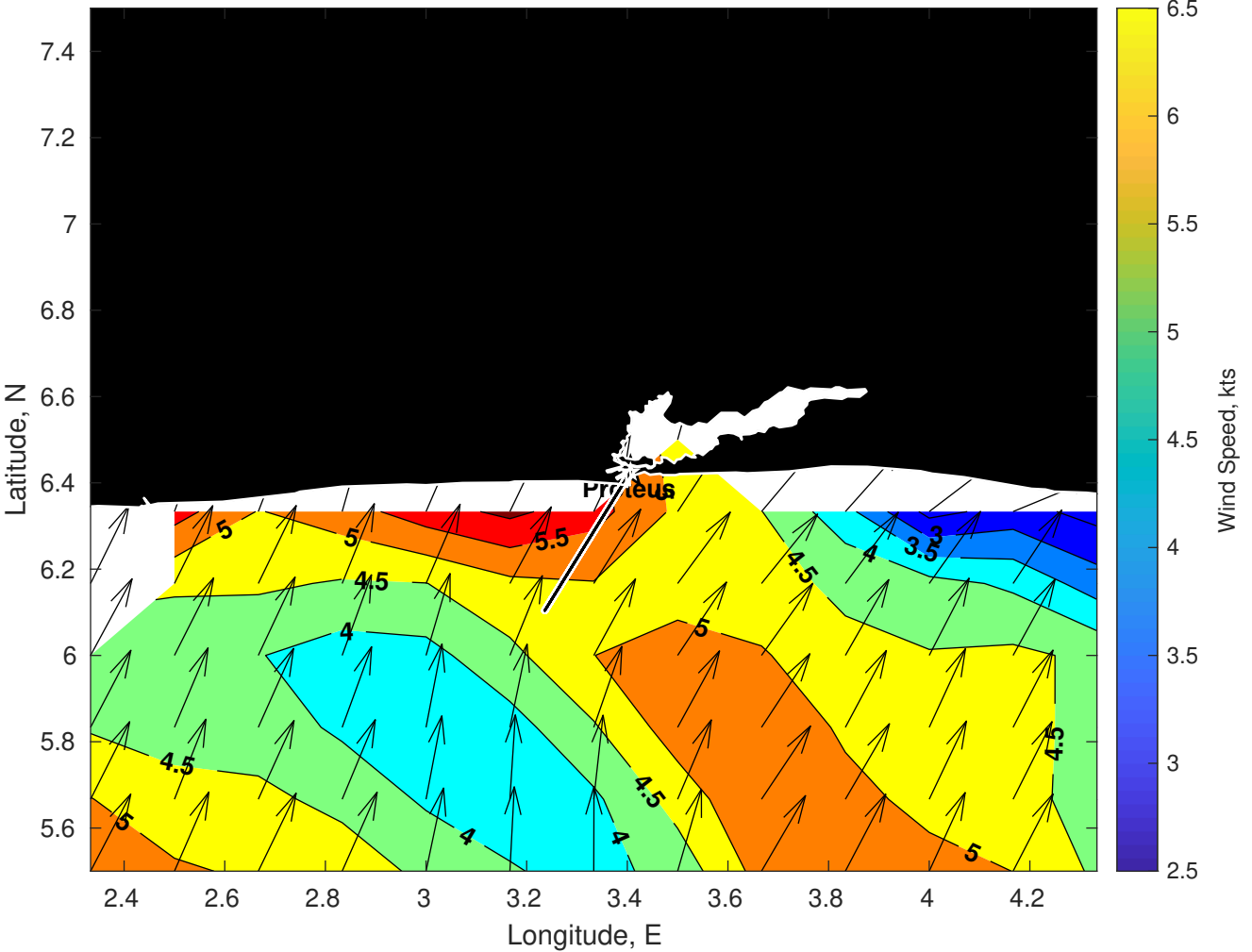
Winds (kts) for Proteus at 17-Oct-2025 09:00:00
