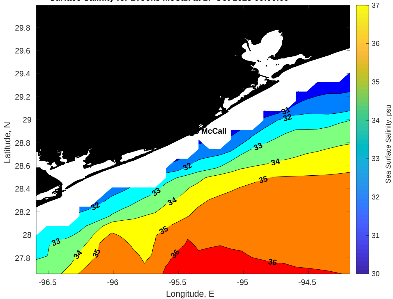
Surface Salinity for Brooks McCall at 17-Oct-2025 00:00:00
