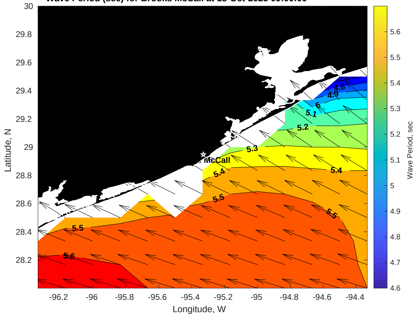
Wave Period (sec) for Brooks McCall at 18-Oct-2025 09:00:00
