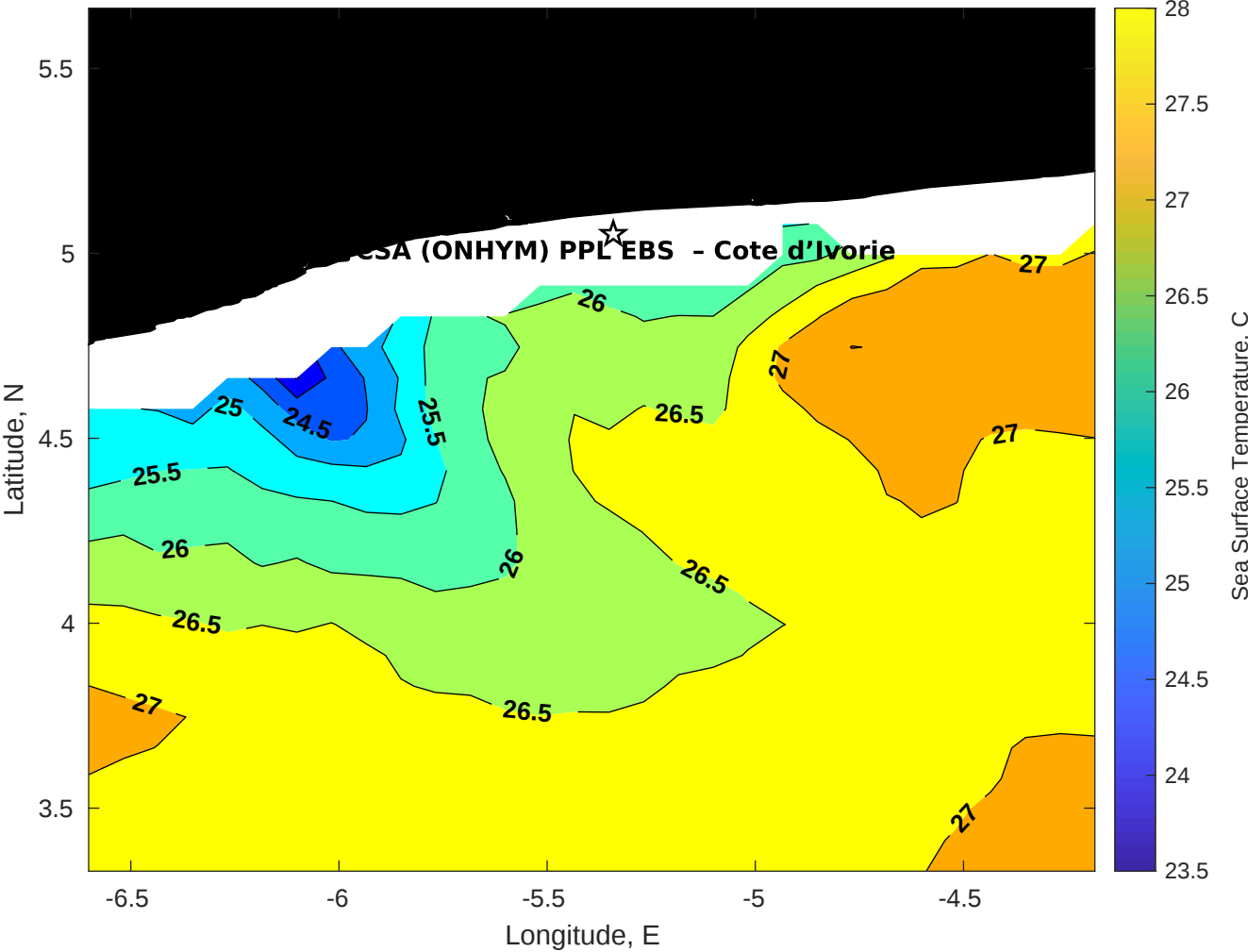
SST for CSA (ONHYM) PPL EBS - Cote d'Ivoire at 17-Oct-2025 00:00:00
