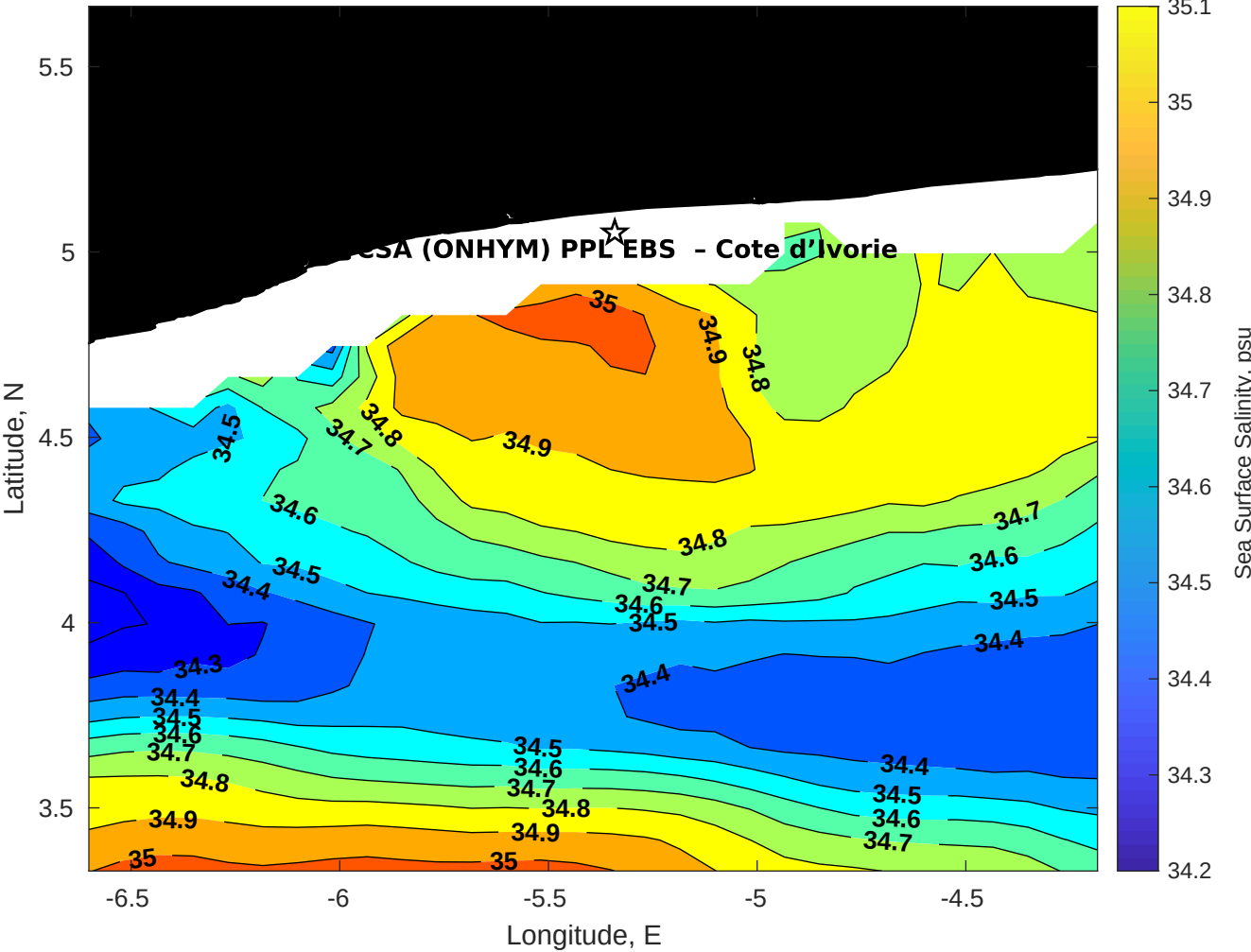
Surface Salinity for CSA (ONHYM) PPL EBS - Cote d'Ivoire at 17-Oct-2025 00:00:00
