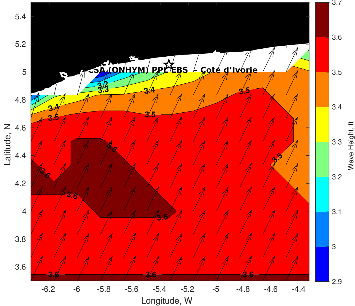
Wave Height (ft) for CSA (ONHYM) PPL EBS - Cote d'Ivoire at 18-Oct-2025 09:00:00
