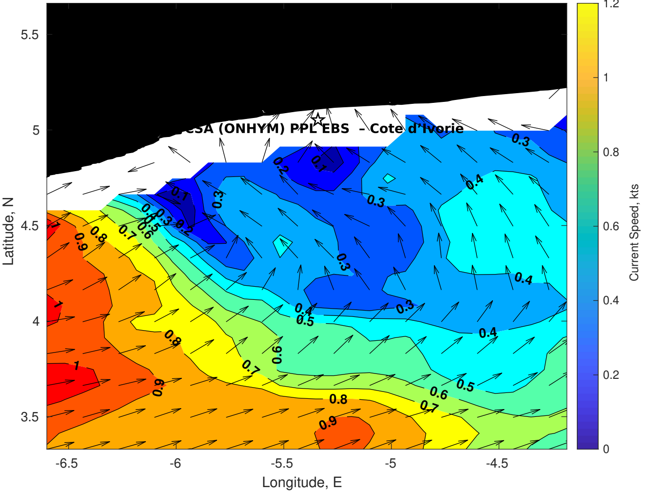
Surface Currents for CSA (ONHYM) PPL EBS - Cote d'Ivoire at 17-Oct-2025 00:00:00
