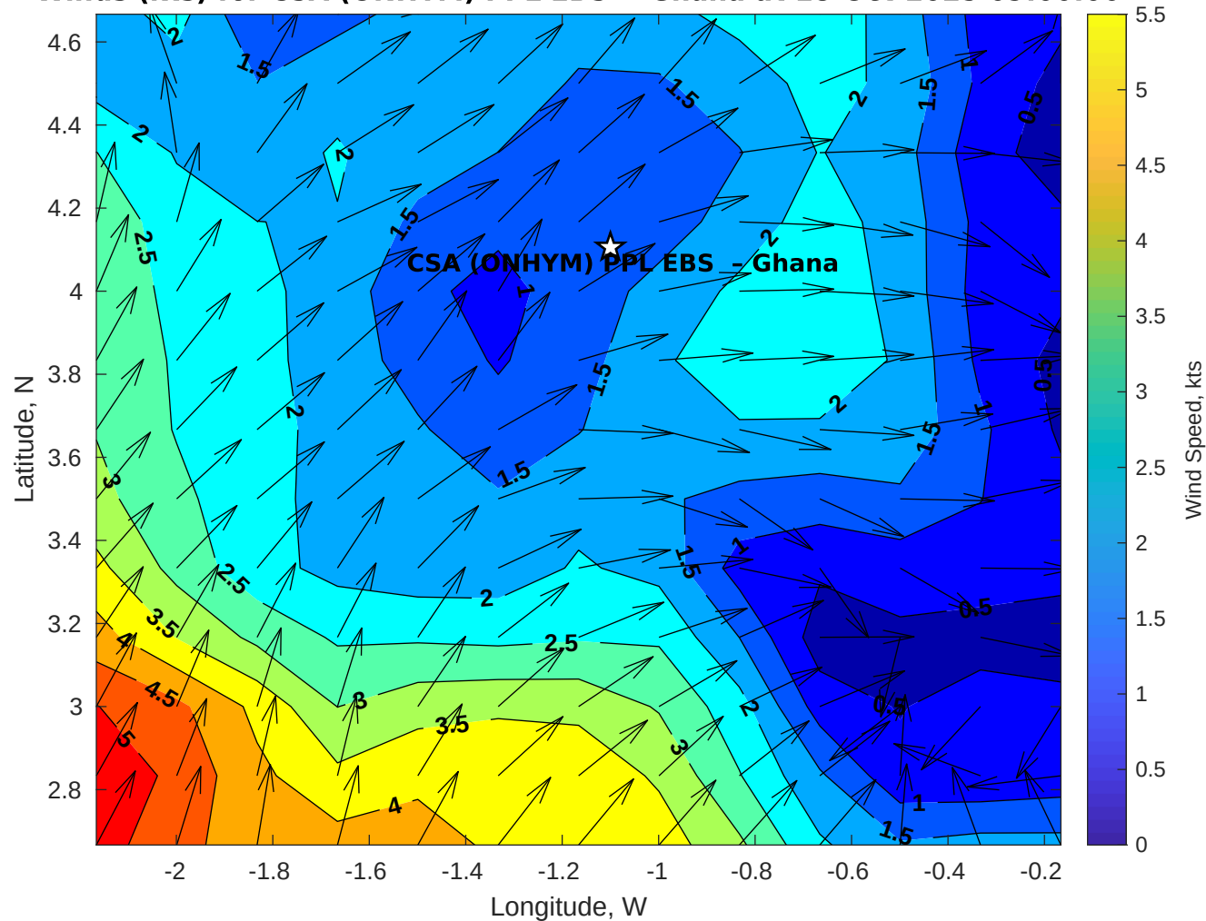
Winds (kts) for CSA (ONHYM) PPL EBS - Ghana at 18-Oct-2025 09:00:00
