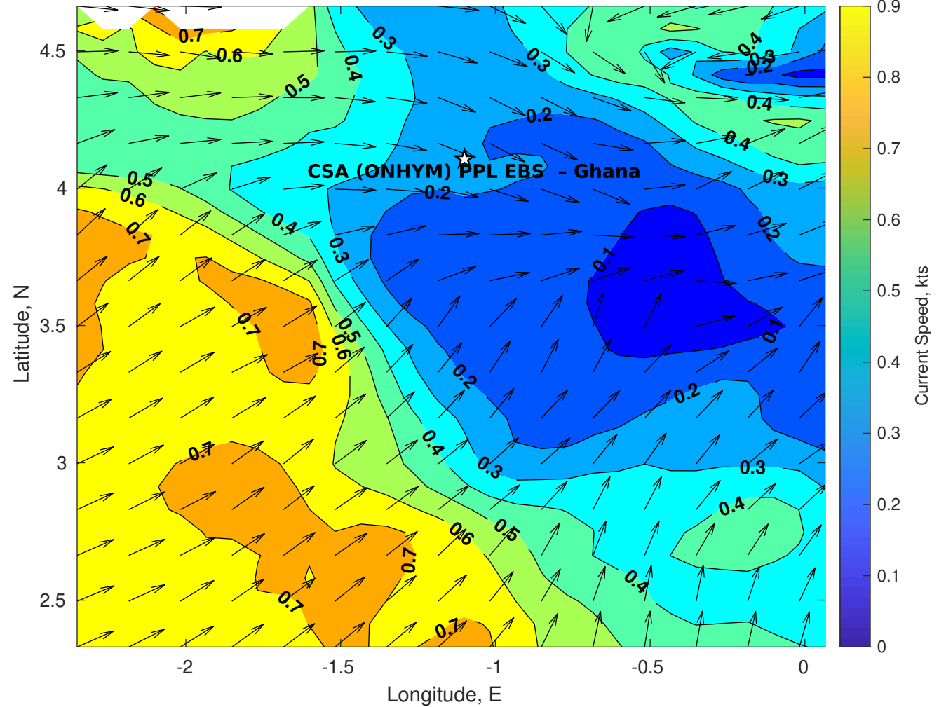
Surface Currents for CSA (ONHYM) PPL EBS - Ghana at 17-Oct-2025 00:00:00
