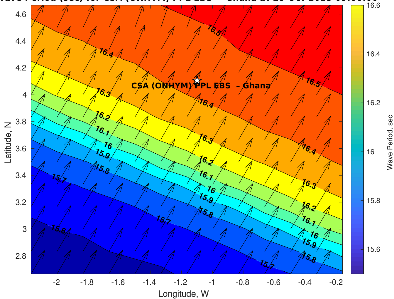
Wave Period (sec) for CSA (ONHYM) PPL EBS - Ghana at 18-Oct-2025 09:00:00
