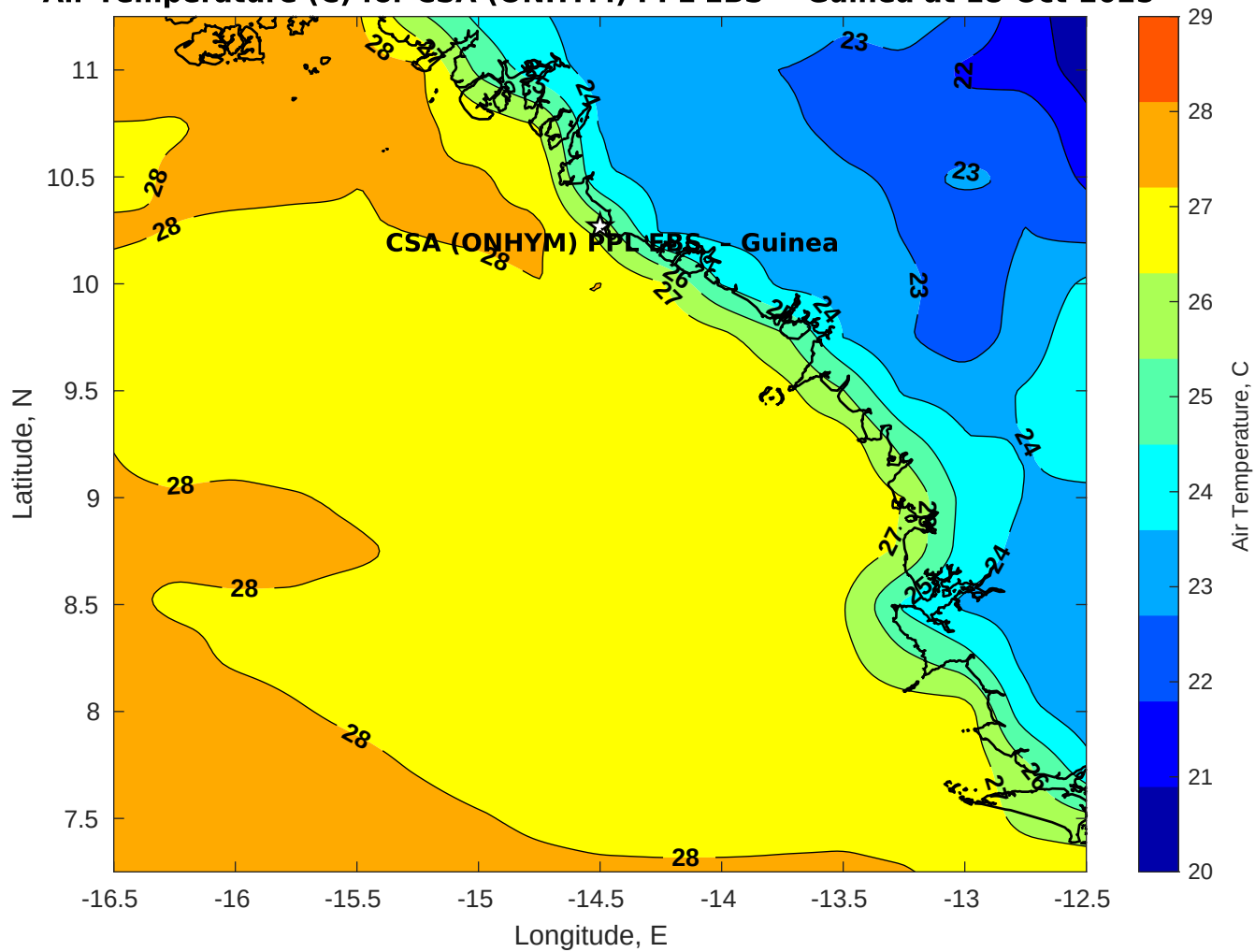
Air Temperature (C) for CSA (ONHYM) PPL EBS - Guinea at 18-Oct-2025
