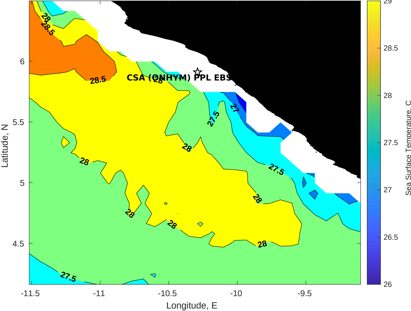
SST for CSA (ONHYM) PPL EBS - Liberia at 17-Oct-2025 00:00:00
