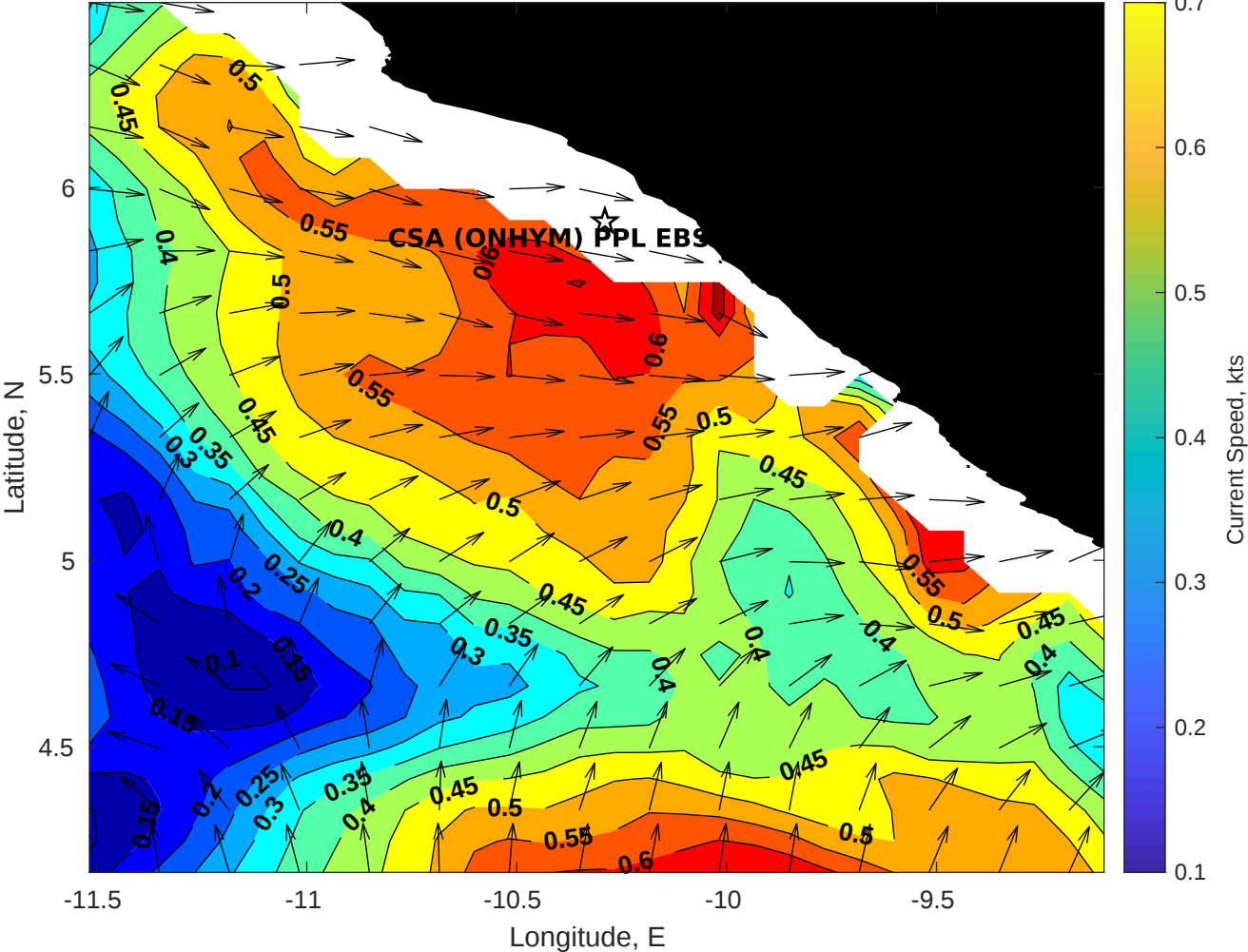
Surface Currents for CSA (ONHYM) PPL EBS - Liberia at 17-Oct-2025 00:00:00
