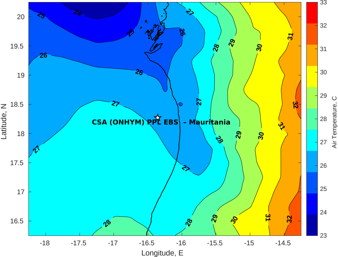
Air Temperature (C) for CSA (ONHYM) PPL EBS - Mauritania at 18-Oct-2025
