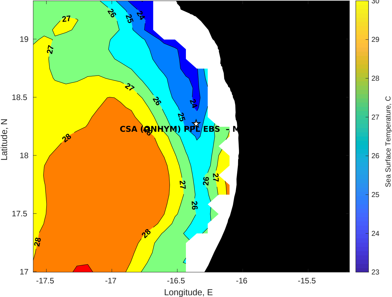
SST for CSA (ONHYM) PPL EBS - Mauritania at 17-Oct-2025 00:00:00
