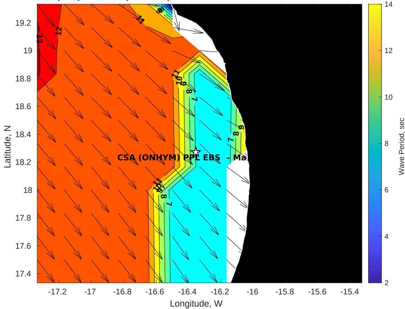
Wave Period (sec) for CSA (ONHYM) PPL EBS - Mauritania at 18-Oct-2025 09:00:00
