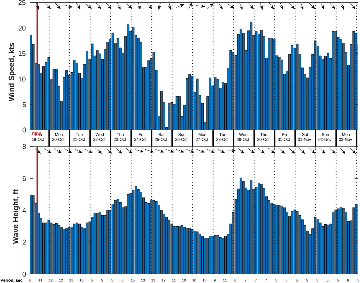
Wind & Wave Forecast for CSA (ONHYM) PPL EBS - Mauritania from 18-Oct-2025 01:00:00 to 03-Nov-2025 01:00:00
