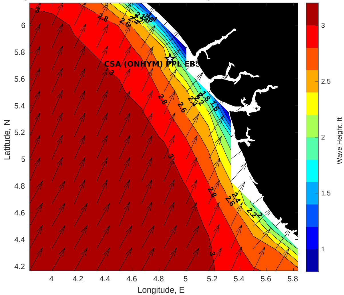
Wave Height (ft) for CSA (ONHYM) PPL EBS - Nigeria at 18-Oct-2025 09:00:00
