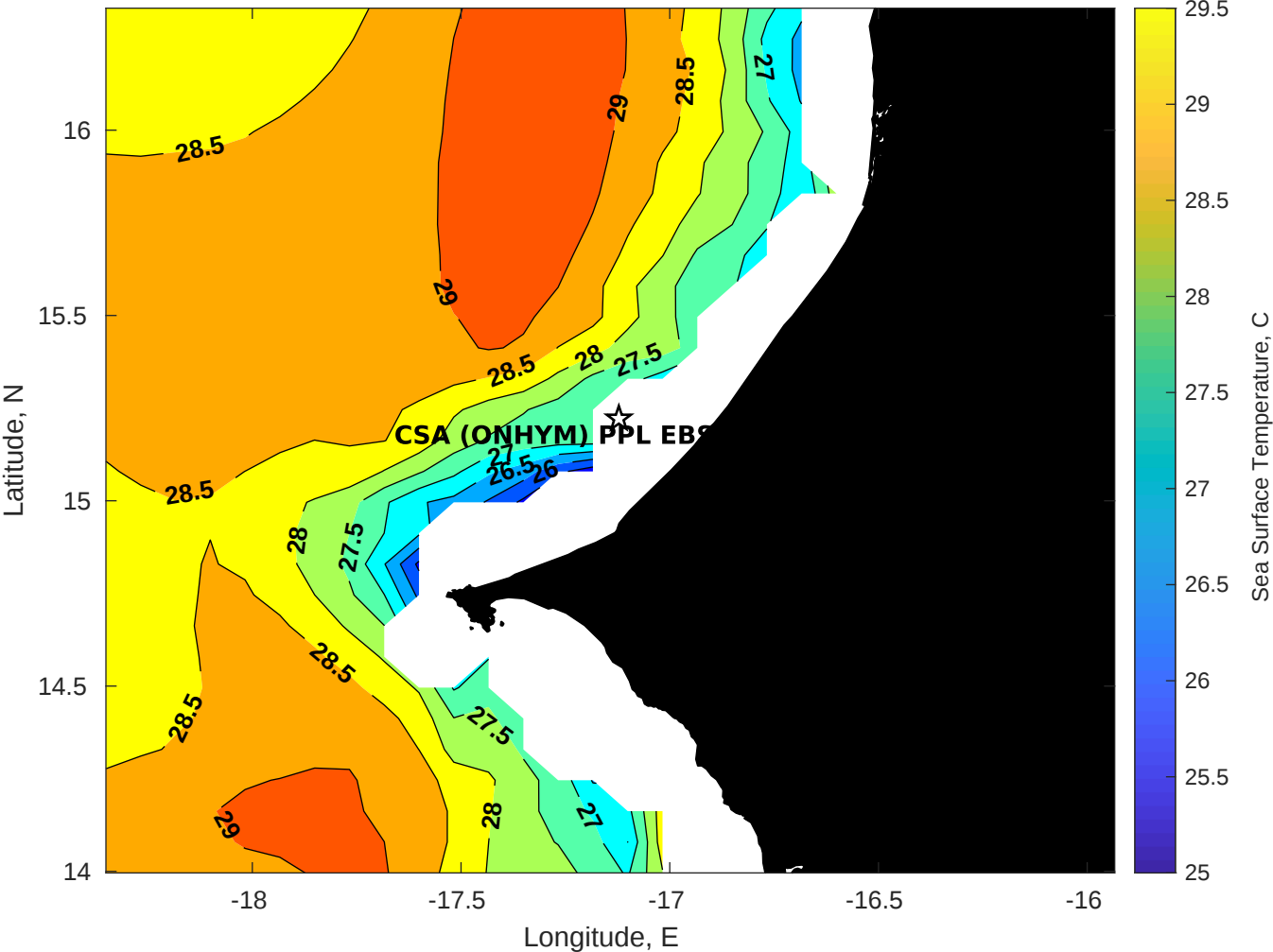
SST for CSA (ONHYM) PPL EBS - Senegal at 17-Oct-2025 00:00:00
