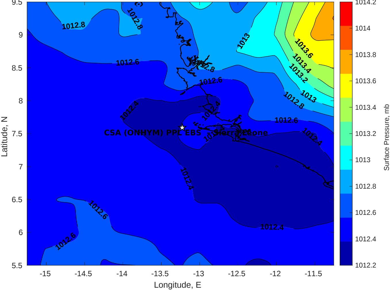
Surface Pressure (mb) for CSA (ONHYM) PPL EBS - Sierra Leone at 18-Oct-2025 00:00:00
