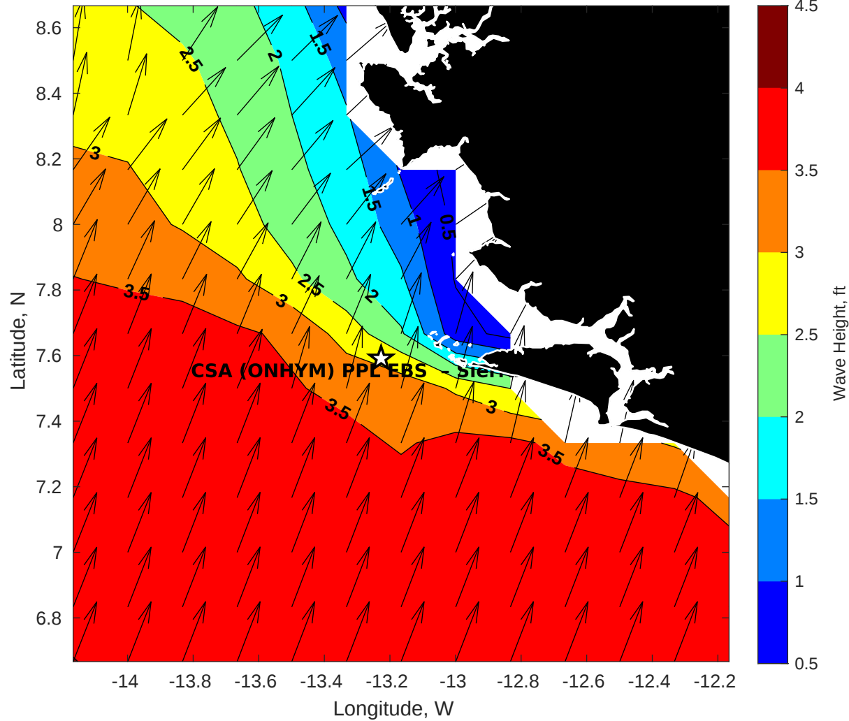
Wave Height (ft) for CSA (ONHYM) PPL EBS - Sierra Leone at 18-Oct-2025 09:00:00
