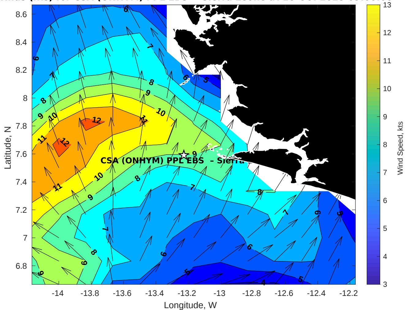
Winds (kts) for CSA (ONHYM) PPL EBS - Sierra Leone at 18-Oct-2025 09:00:00
