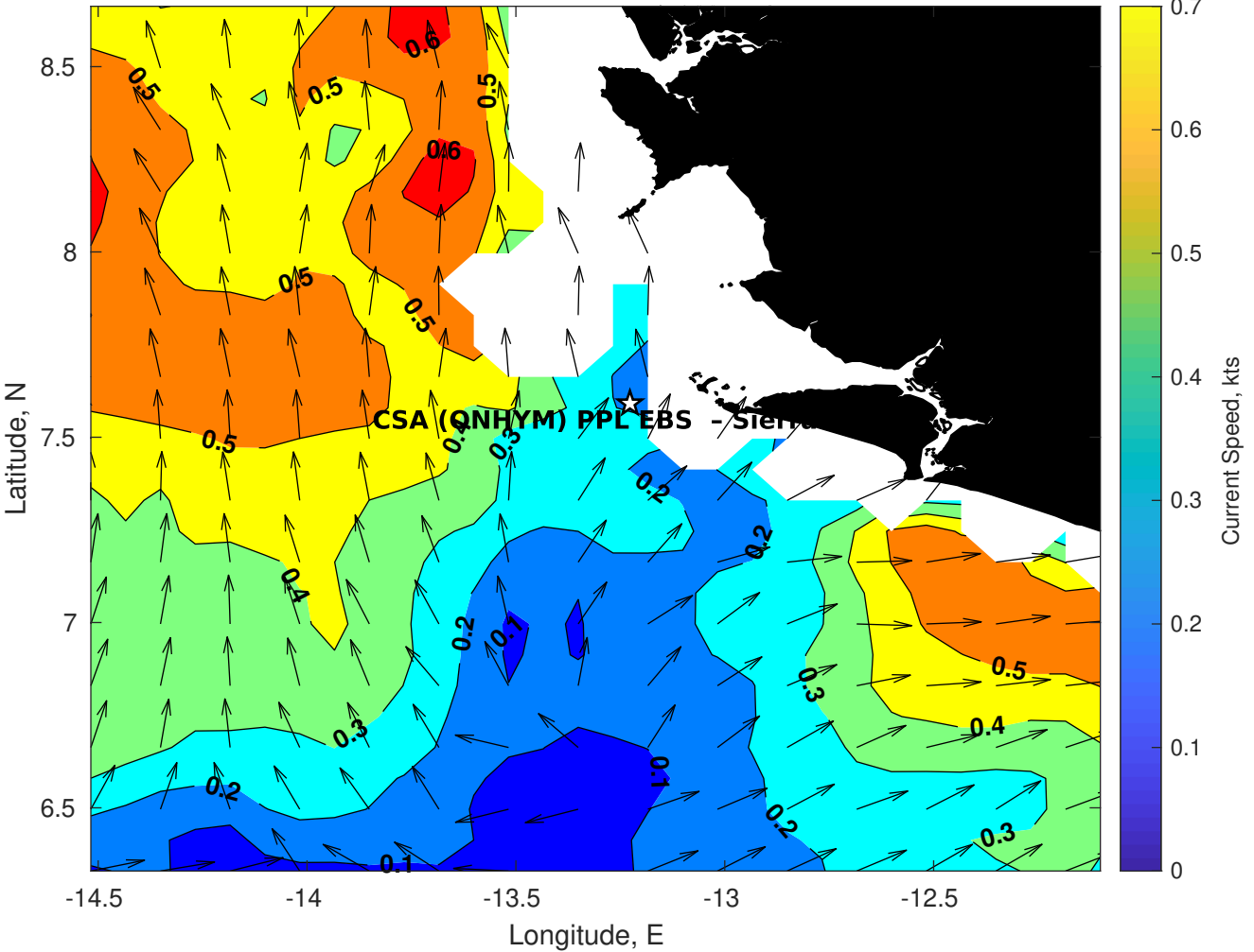
Surface Currents for CSA (ONHYM) PPL EBS - Sierra Leone at 17-Oct-2025 00:00:00
