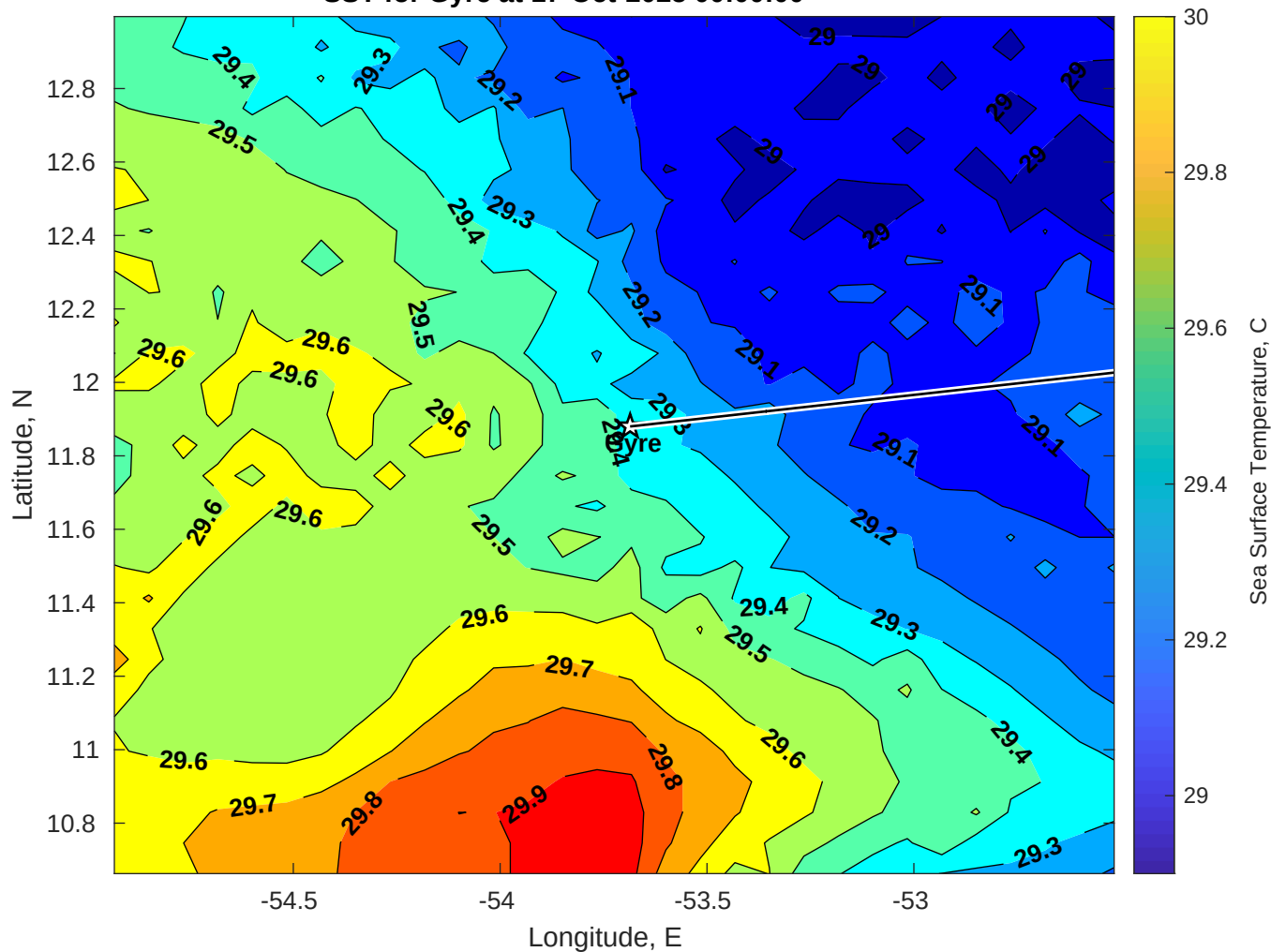
SST for Gyre at 17-Oct-2025 00:00:00
