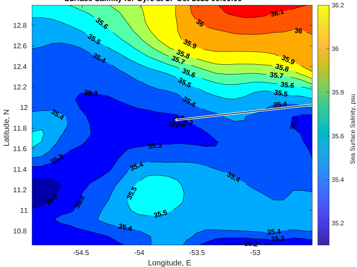
Surface Salinity for Gyre at 17-Oct-2025 00:00:00
