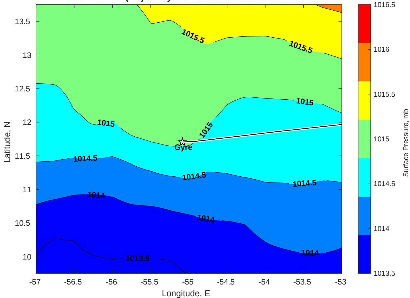
Surface Pressure (mb) for Gyre at 20-Oct-2025 00:00:00
