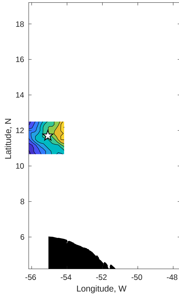
World View - Gyre
