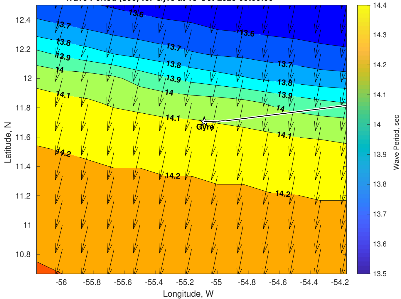
Wave Period (sec) for Gyre at 18-Oct-2025 09:00:00
