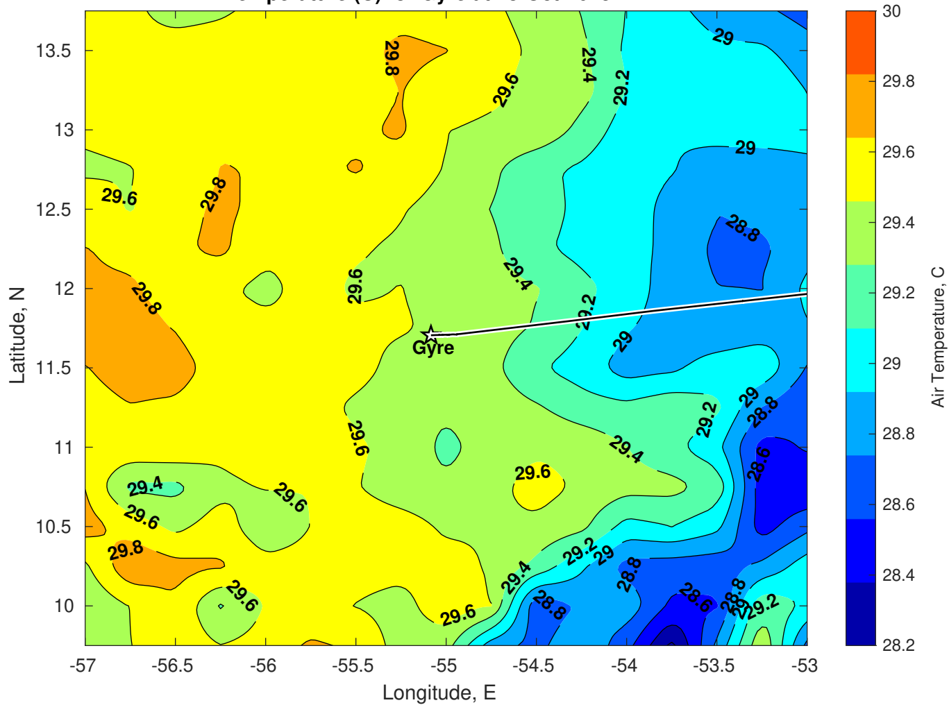
Air Temperature (C) for Gyre at 18-Oct-2025
