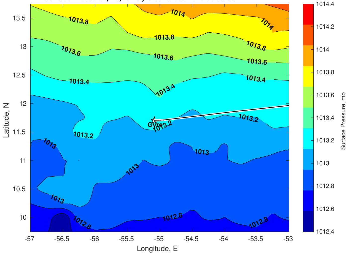
Surface Pressure (mb) for Gyre at 18-Oct-2025 00:00:00
