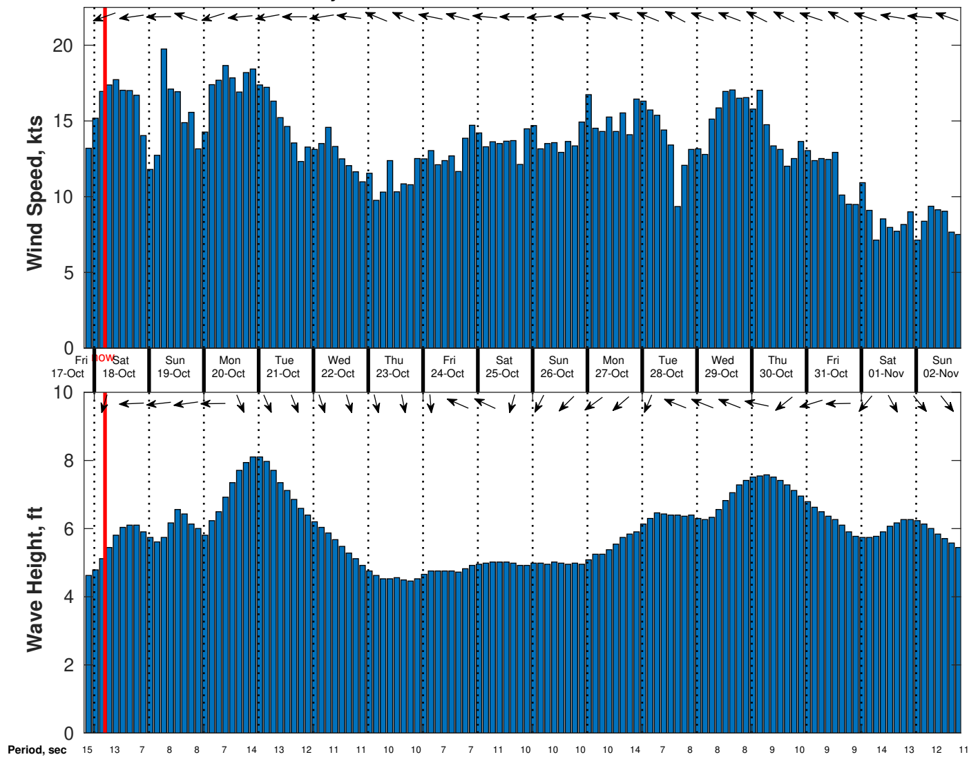
Wind & Wave Forecast for Gyre from 17-Oct-2025 20:00:00 to 02-Nov-2025 20:00:00
