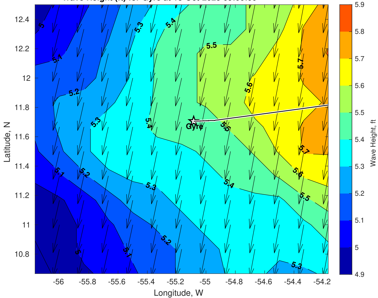
Wave Height (ft) for Gyre at 18-Oct-2025 09:00:00
