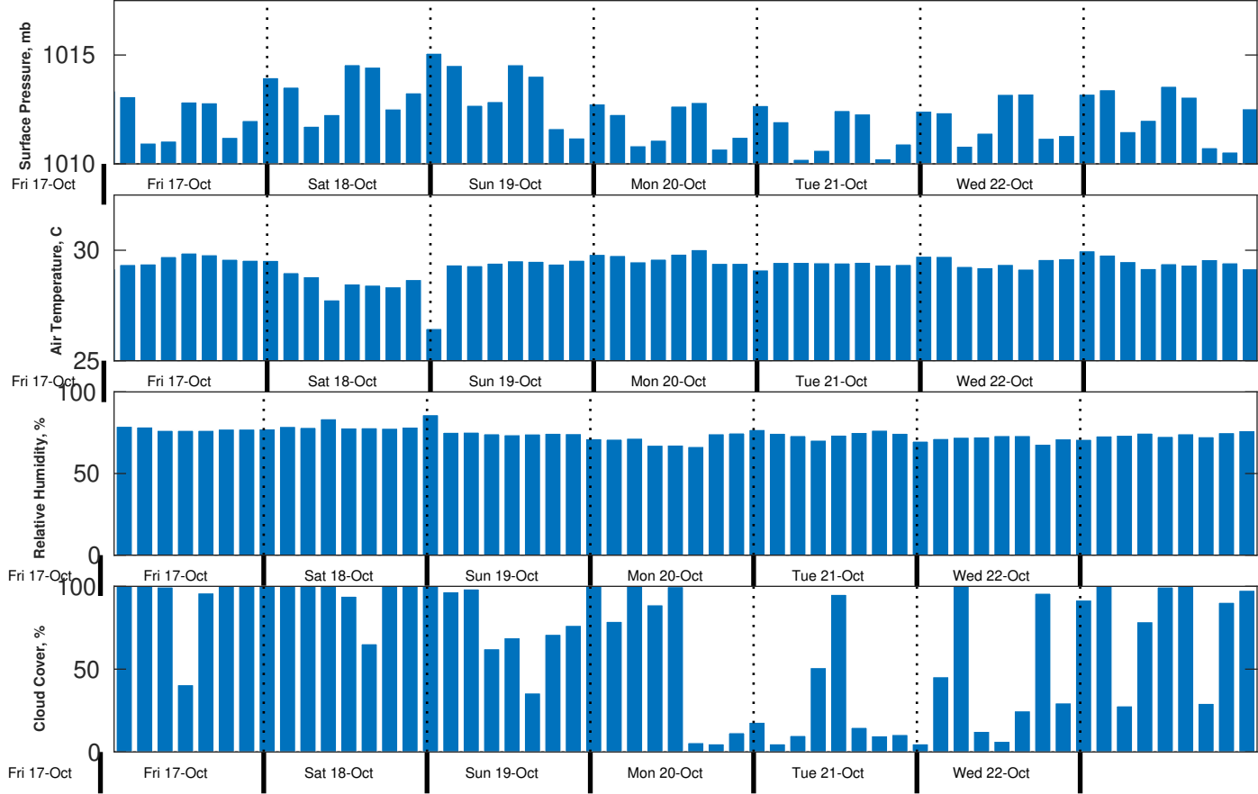
Met Forecast for Gyre from 17-Oct-2025 20:00:00 to 24-Oct-2025 20:00:00
