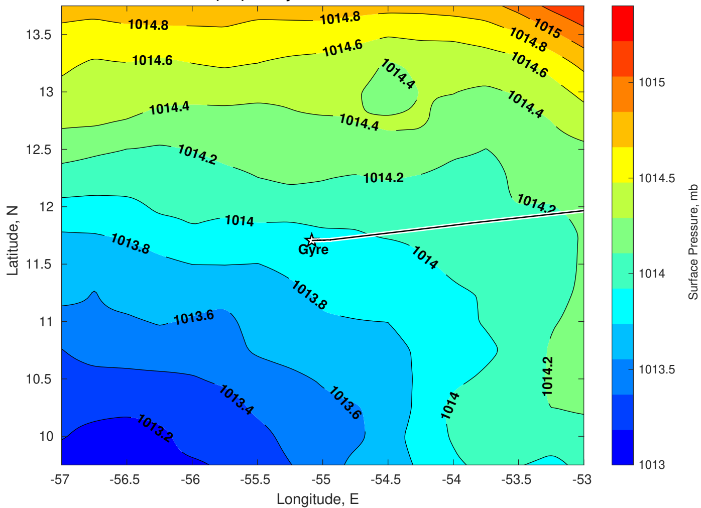
Surface Pressure (mb) for Gyre at 19-Oct-2025 00:00:00
