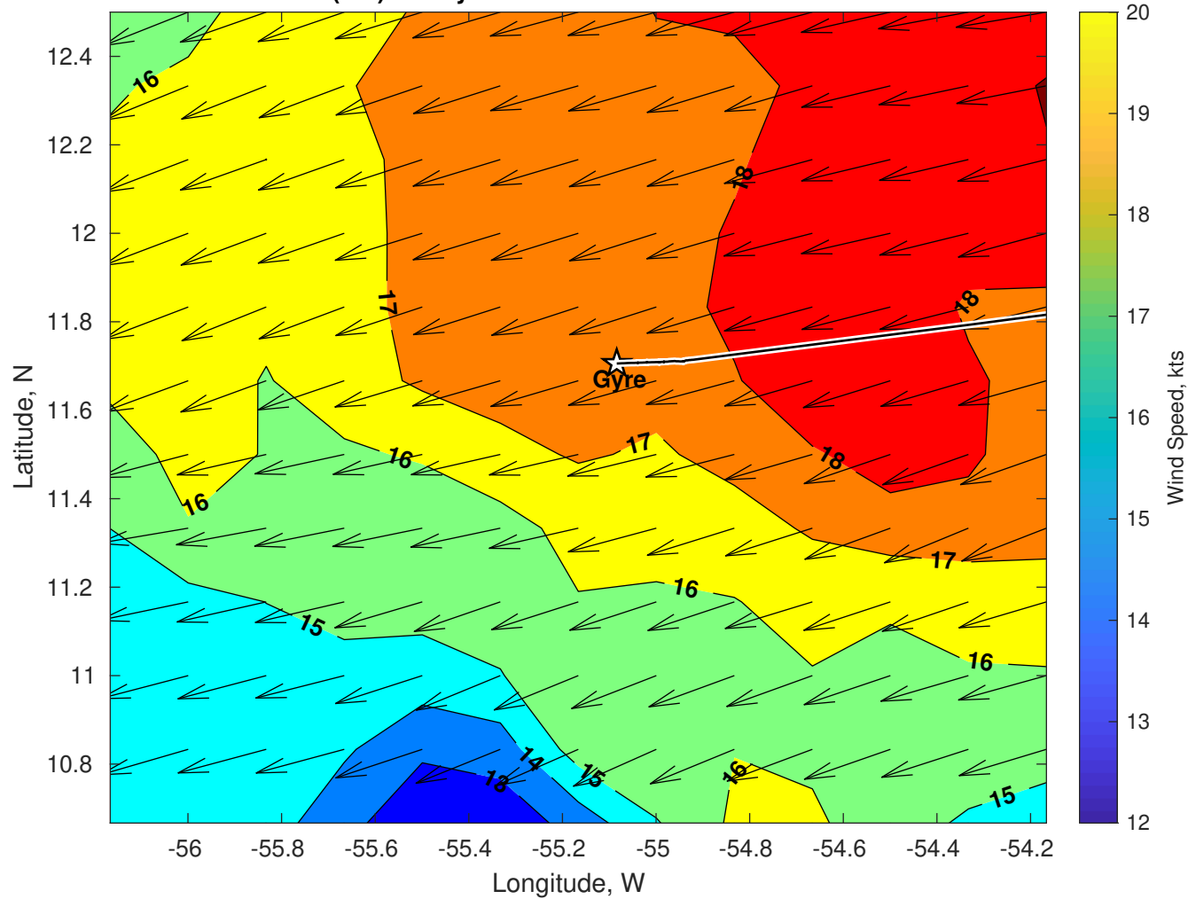
Winds (kts) for Gyre at 18-Oct-2025 09:00:00
