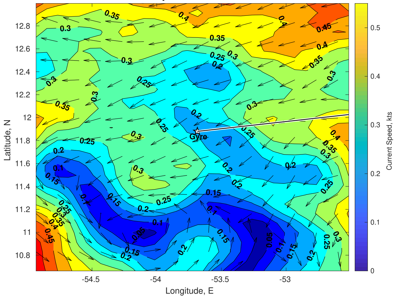
Surface Currents for Gyre at 17-Oct-2025 00:00:00
