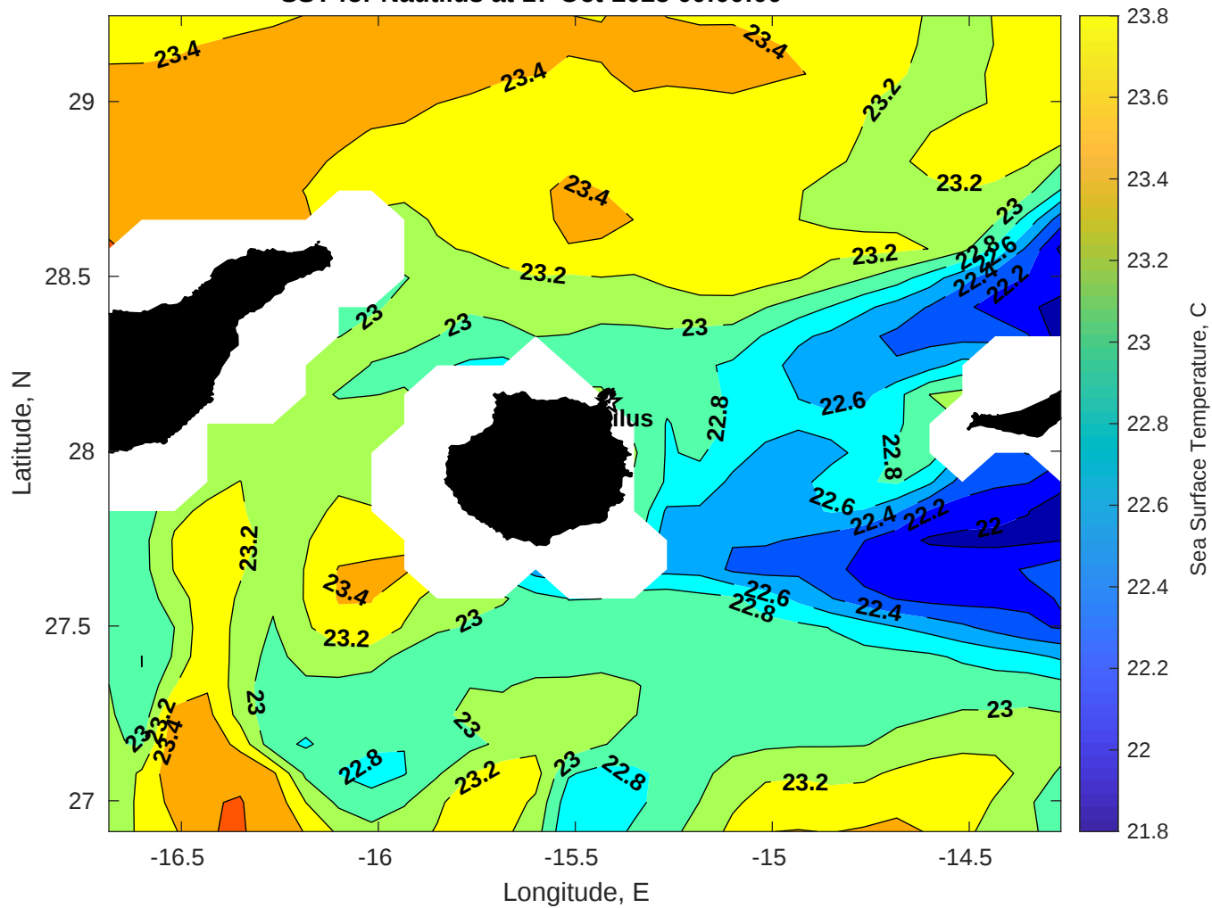
SST for Nautilus at 17-Oct-2025 00:00:00
