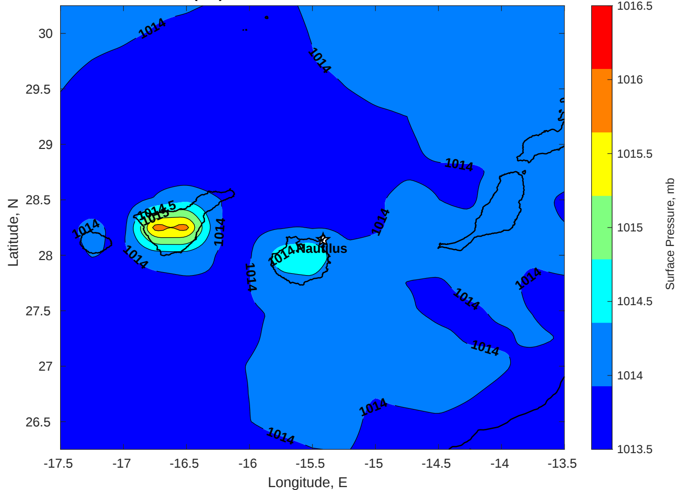
Surface Pressure (mb) for Nautilus at 18-Oct-2025 00:00:00
