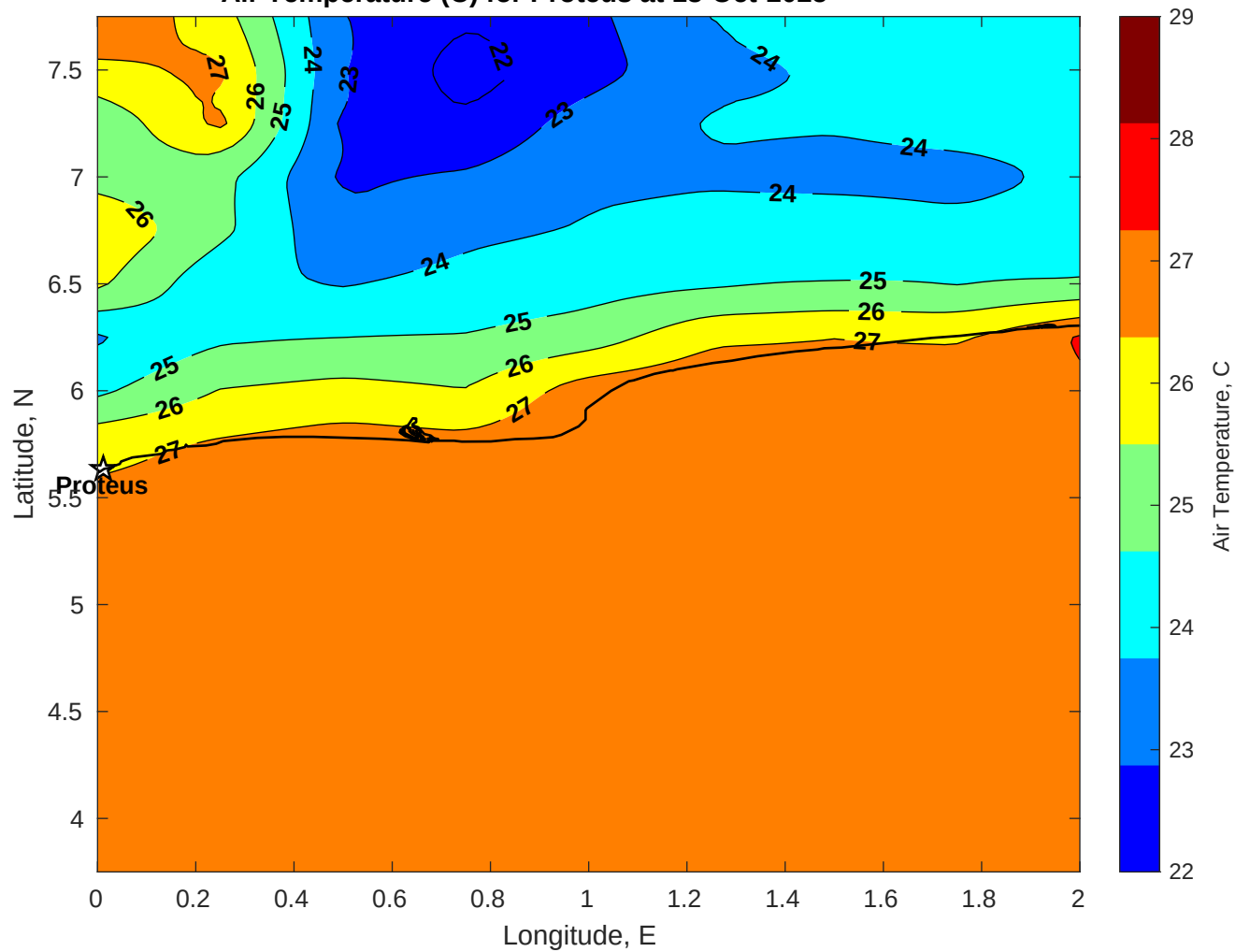
Air Temperature (C) for Proteus at 18-Oct-2025
