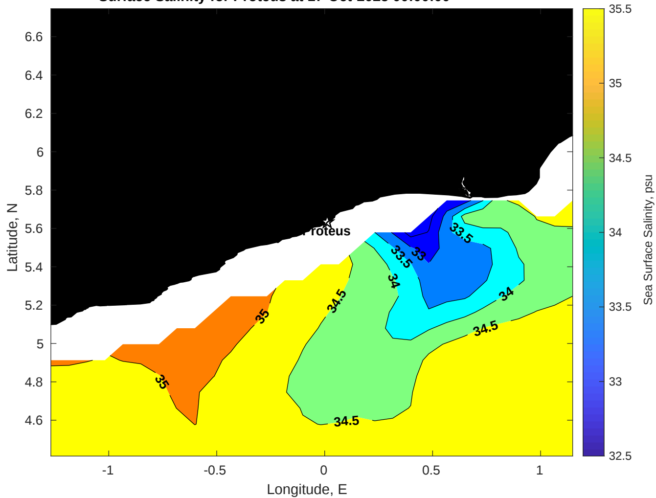
Surface Salinity for Proteus at 17-Oct-2025 00:00:00
