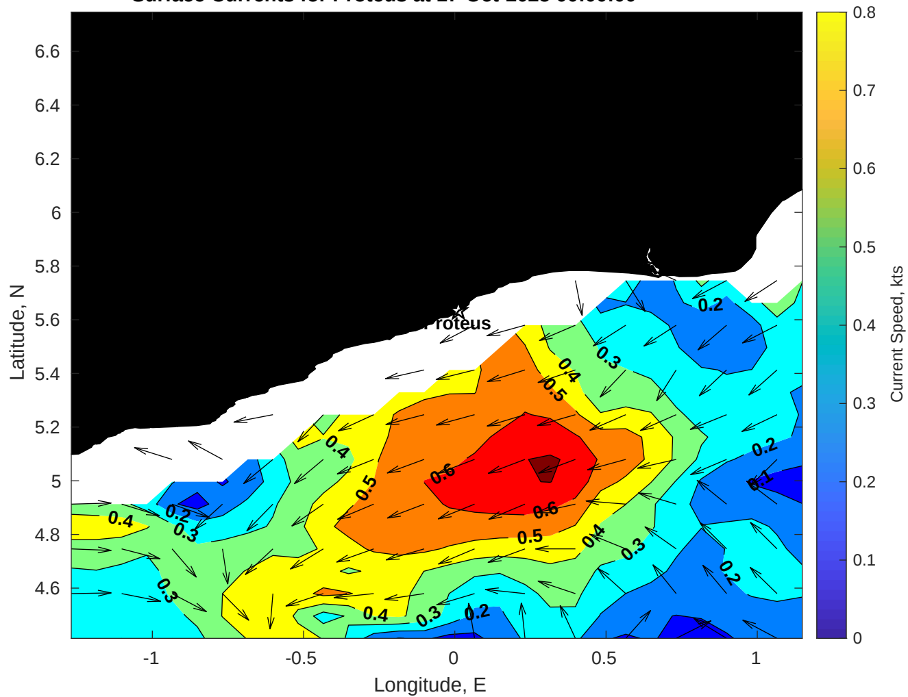
Surface Currents for Proteus at 17-Oct-2025 00:00:00
