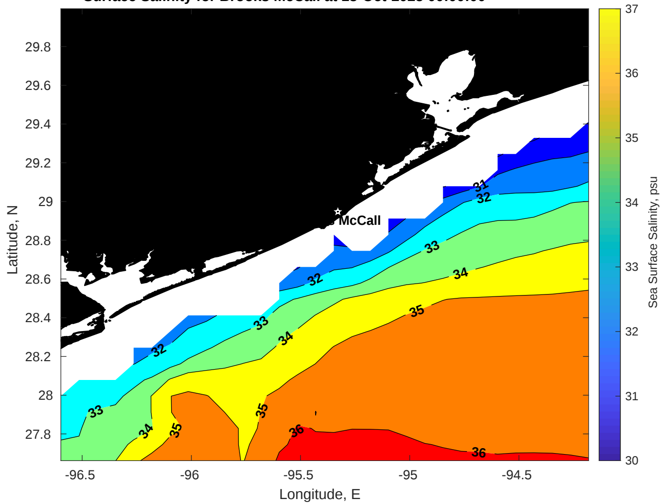
Surface Salinity for Brooks McCall at 18-Oct-2025 00:00:00
