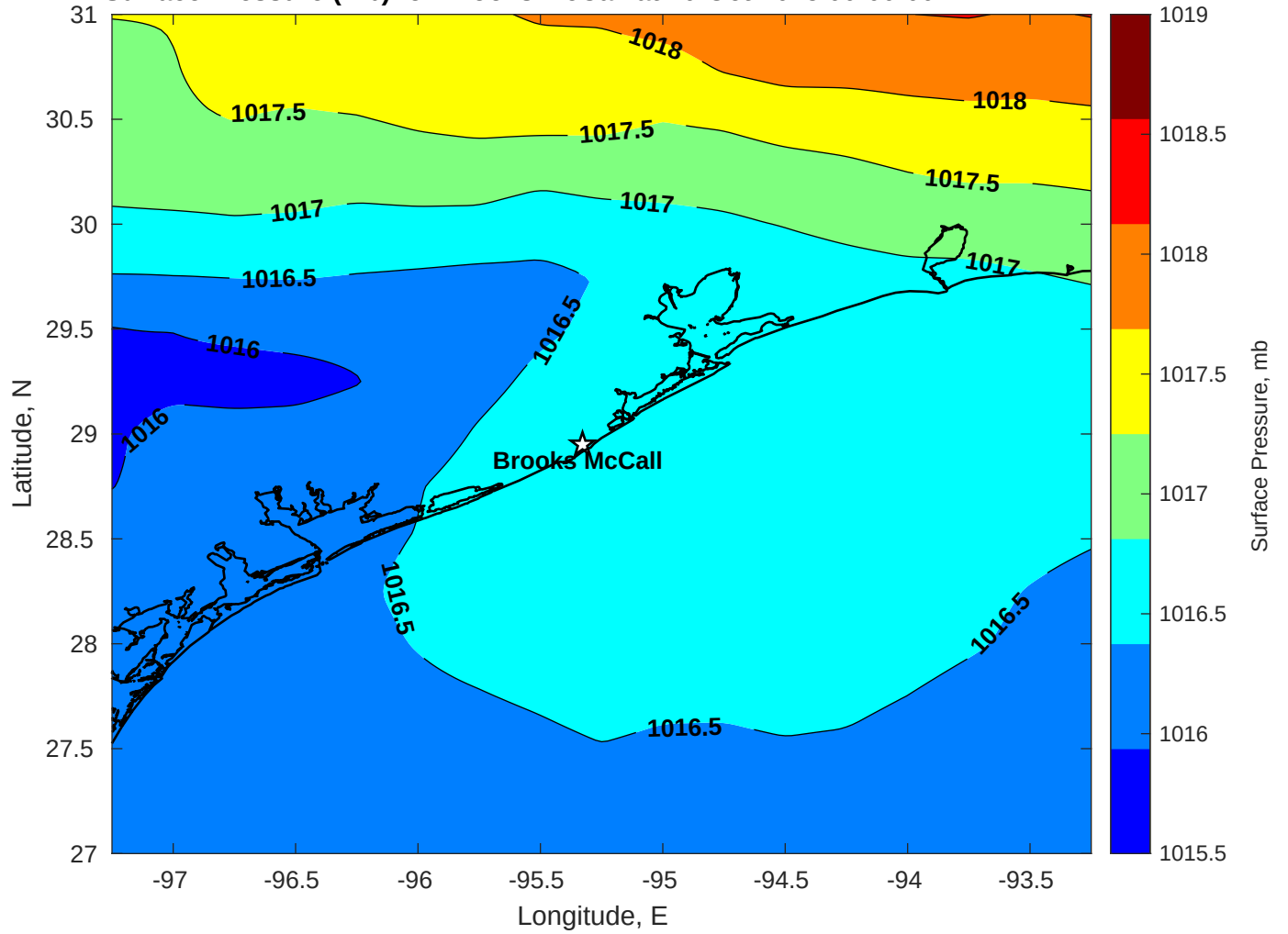
Surface Pressure (mb) for Brooks McCall at 20-Oct-2025 00:00:00
