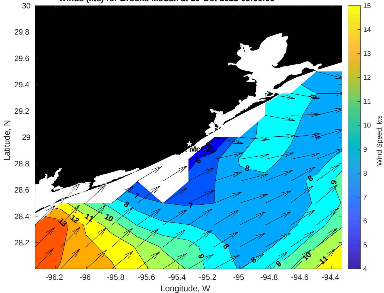
Winds (kts) for Brooks McCall at 19-Oct-2025 09:00:00
