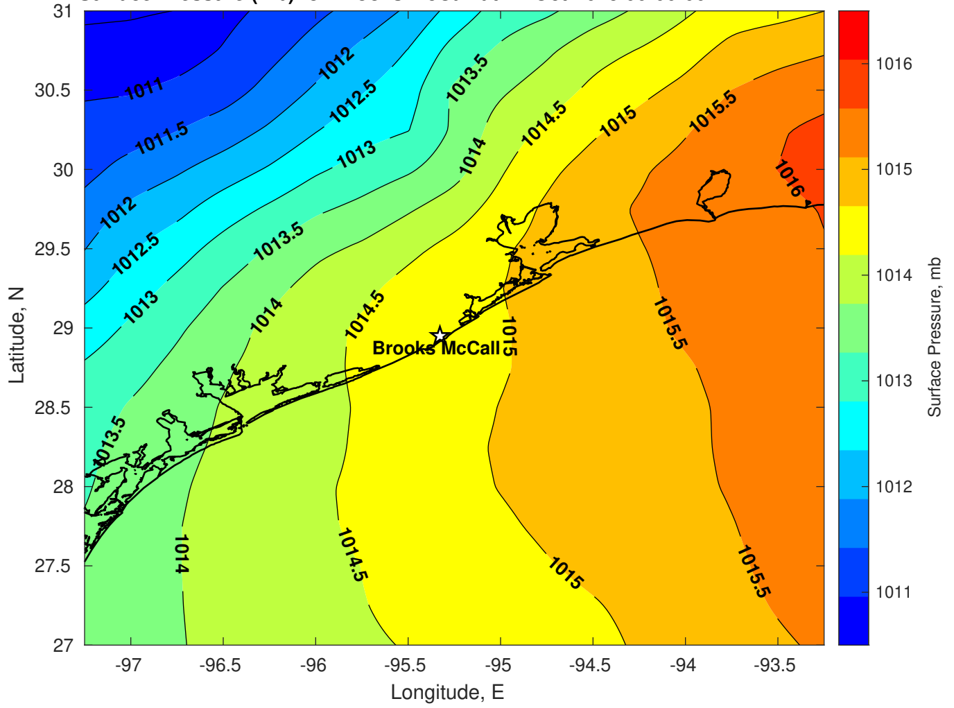
Surface Pressure (mb) for Brooks McCall at 21-Oct-2025 00:00:00
