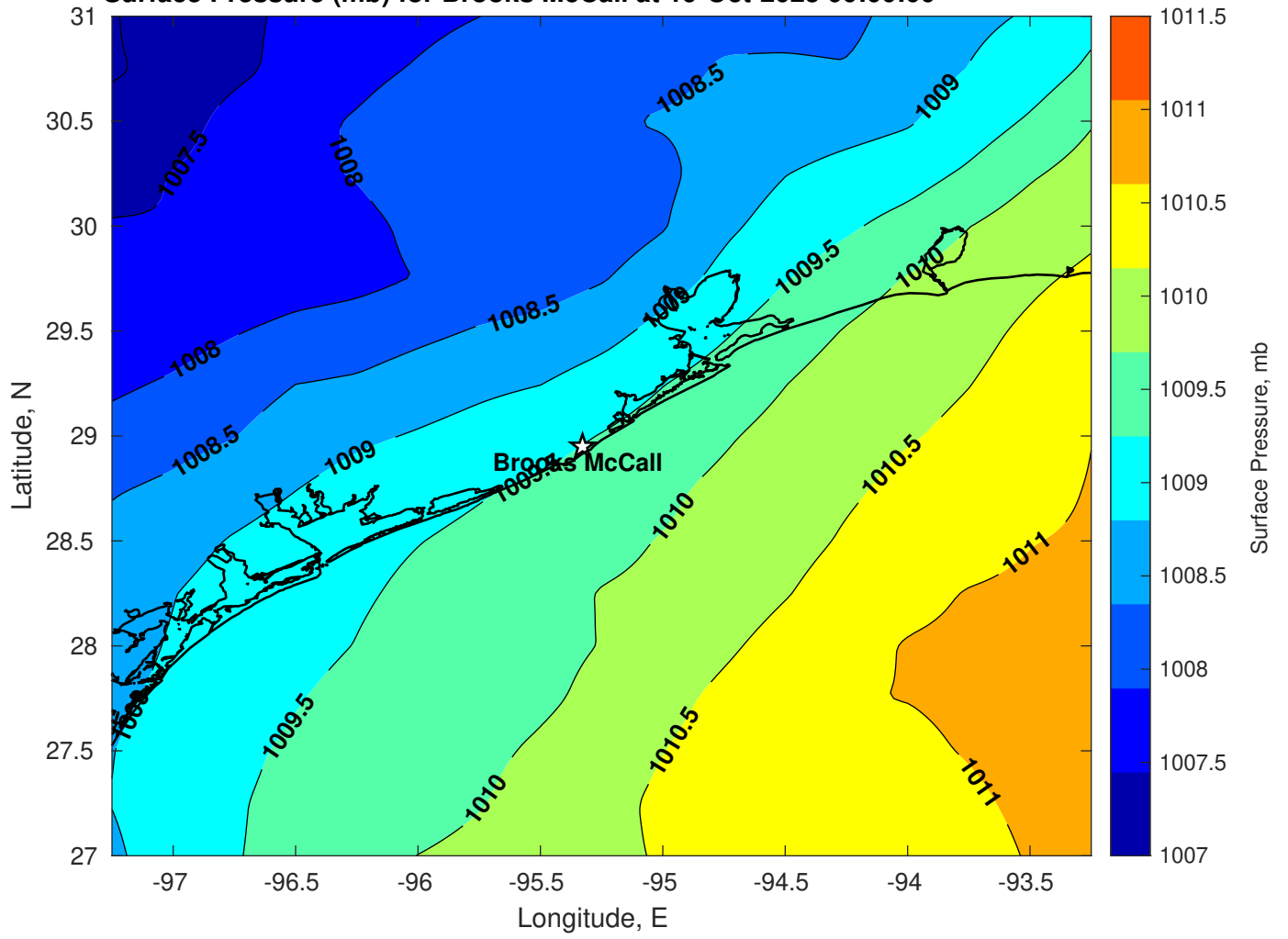
Surface Pressure (mb) for Brooks McCall at 19-Oct-2025 00:00:00
