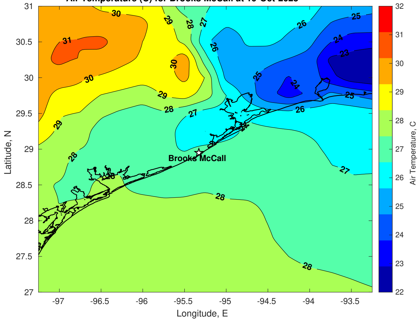
Air Temperature (C) for Brooks McCall at 19-Oct-2025
