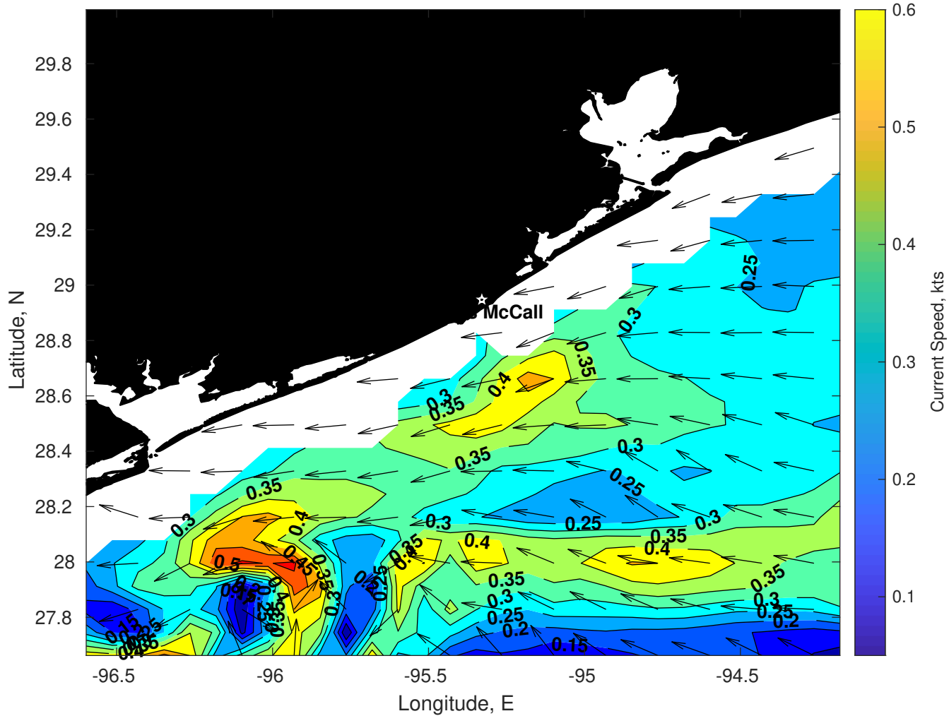
Surface Currents for Brooks McCall at 18-Oct-2025 00:00:00
