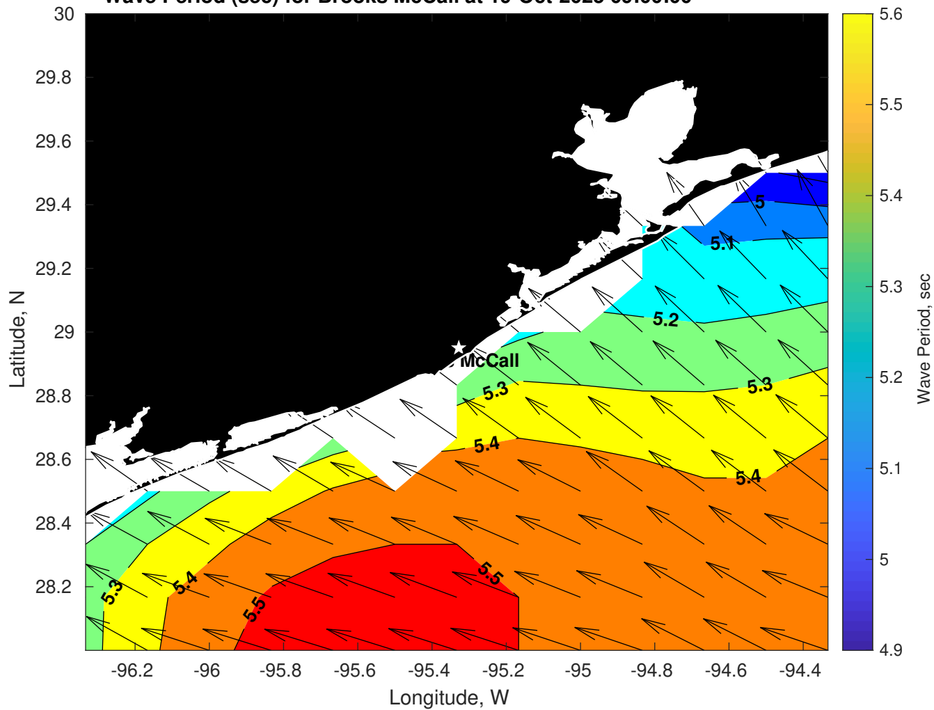
Wave Period (sec) for Brooks McCall at 19-Oct-2025 09:00:00
