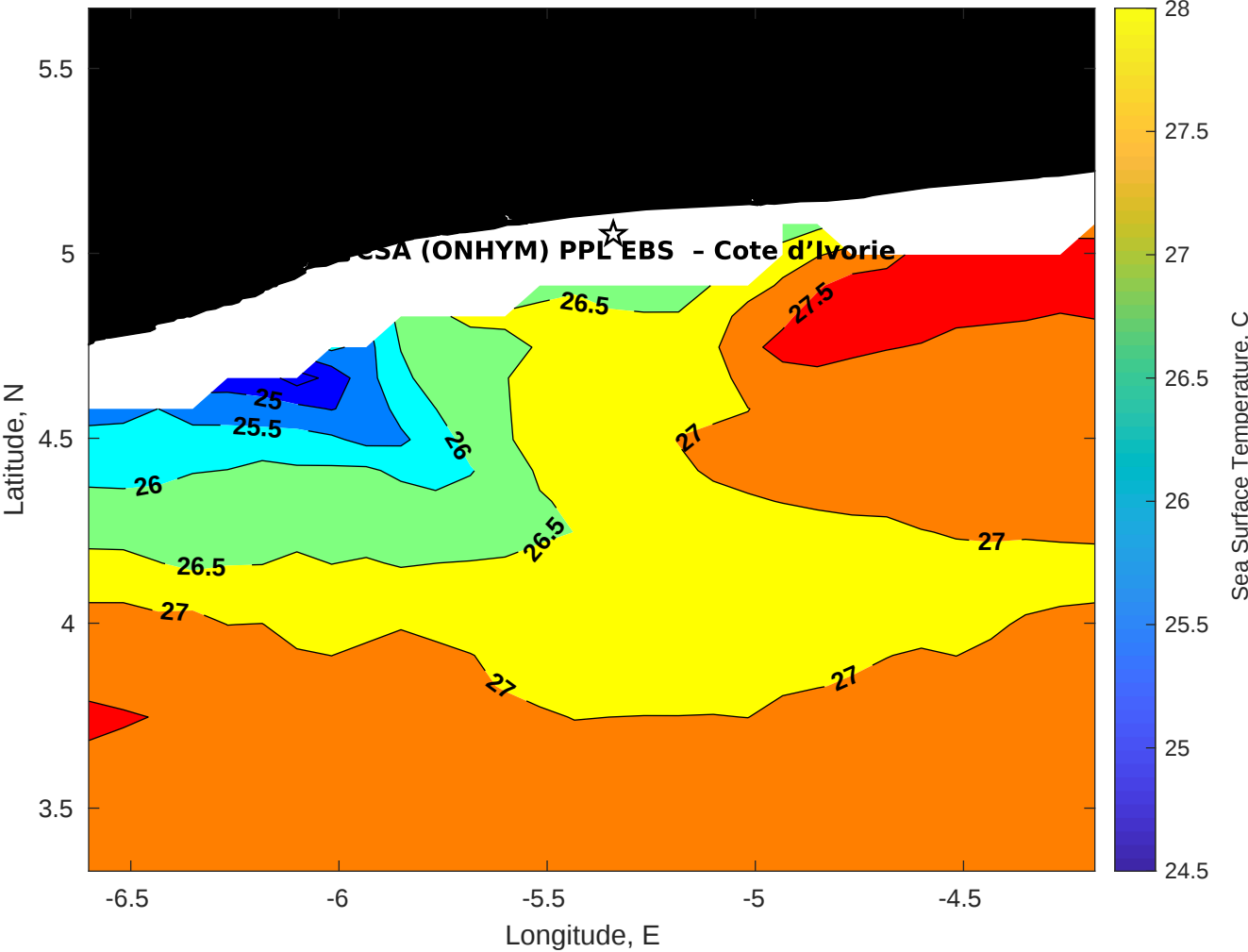
SST for CSA (ONHYM) PPL EBS - Cote d'Ivoire at 18-Oct-2025 00:00:00
