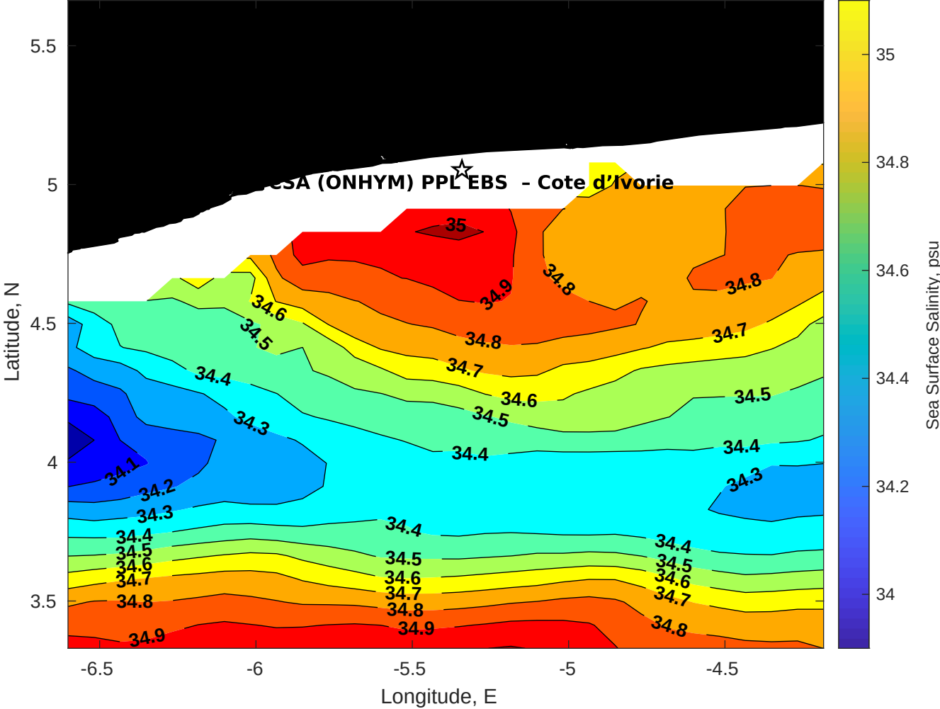
Surface Salinity for CSA (ONHYM) PPL EBS - Cote d'Ivoire at 18-Oct-2025 00:00:00
