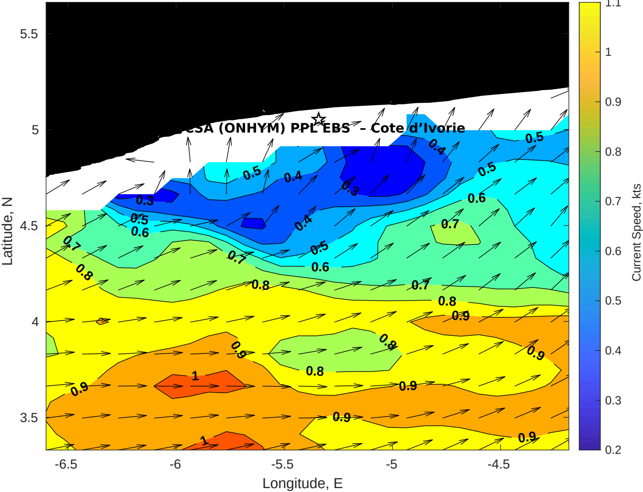
Surface Currents for CSA (ONHYM) PPL EBS - Cote d'Ivoire at 18-Oct-2025 00:00:00
