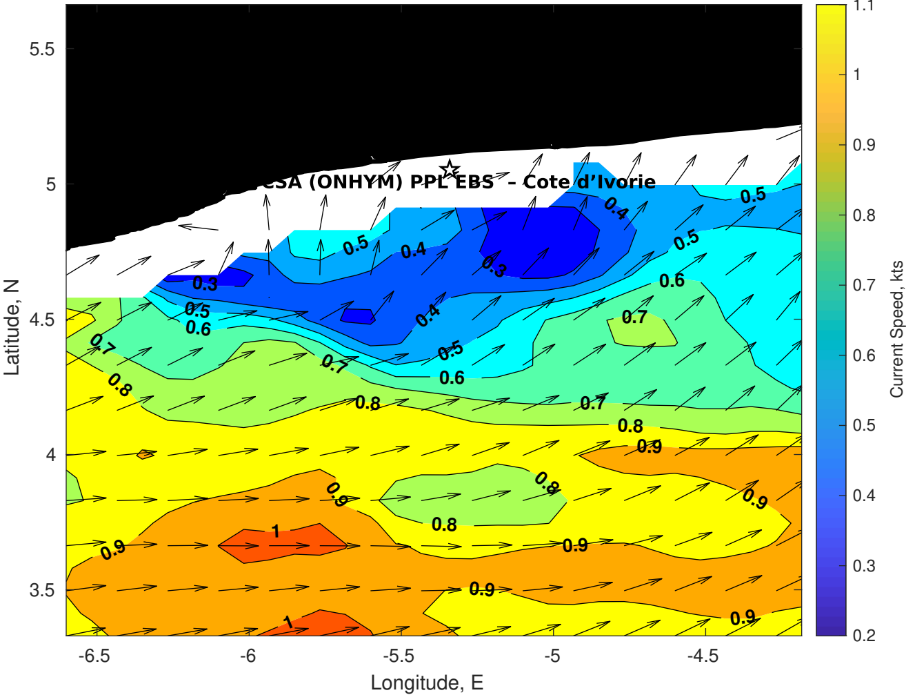
Surface Currents for CSA (ONHYM) PPL EBS - Cote d'Ivoire at 18-Oct-2025 00:00:00
