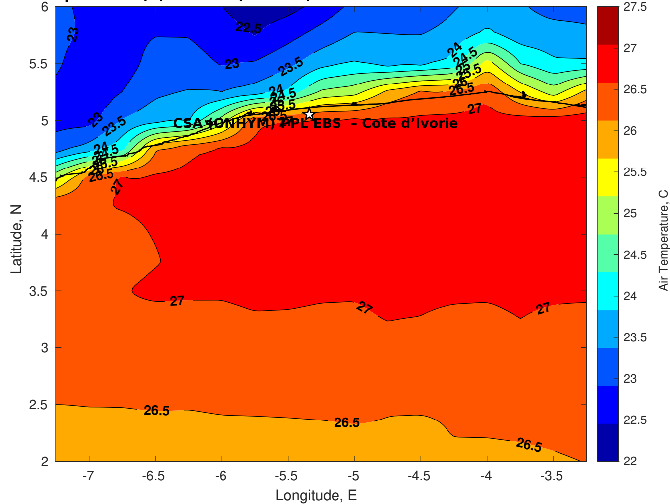
Air Temperature (C) for CSA (ONHYM) PPL EBS - Cote d'Ivoire at 19-Oct-2025
