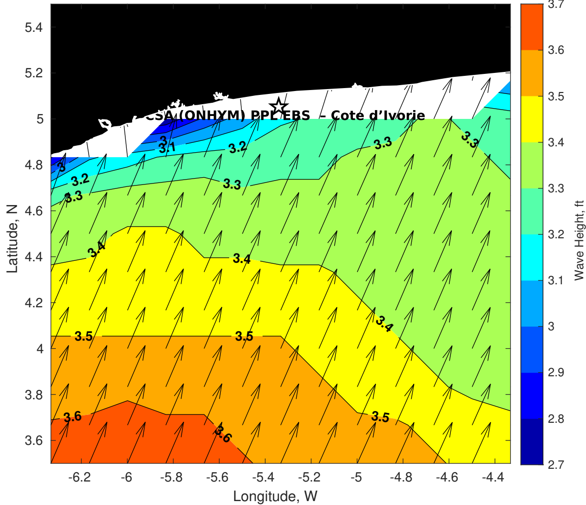
Wave Height (ft) for CSA (ONHYM) PPL EBS - Cote d'Ivoire at 19-Oct-2025 09:00:00
