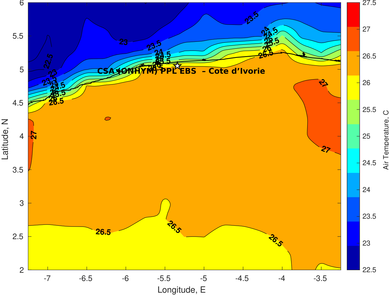
Air Temperature (C) for CSA (ONHYM) PPL EBS - Cote d'Ivoire at 19-Oct-2025
