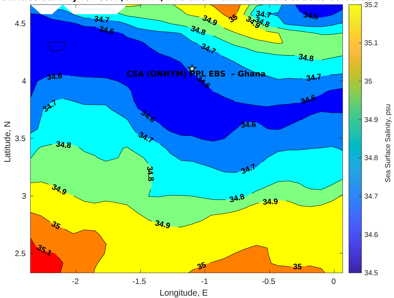
Surface Salinity for CSA (ONHYM) PPL EBS - Ghana at 18-Oct-2025 00:00:00
