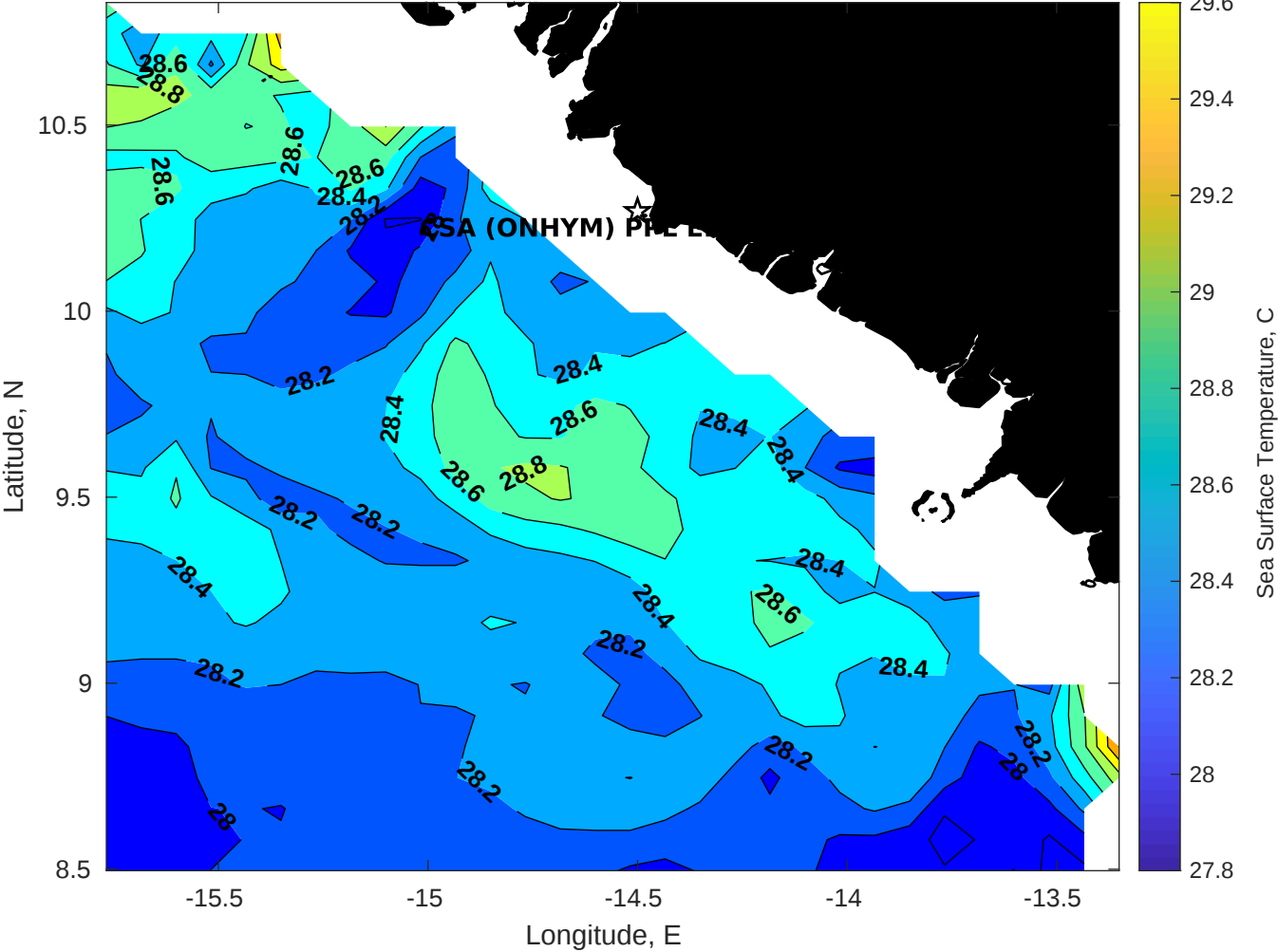
SST for CSA (ONHYM) PPL EBS - Guinea at 18-Oct-2025 00:00:00
