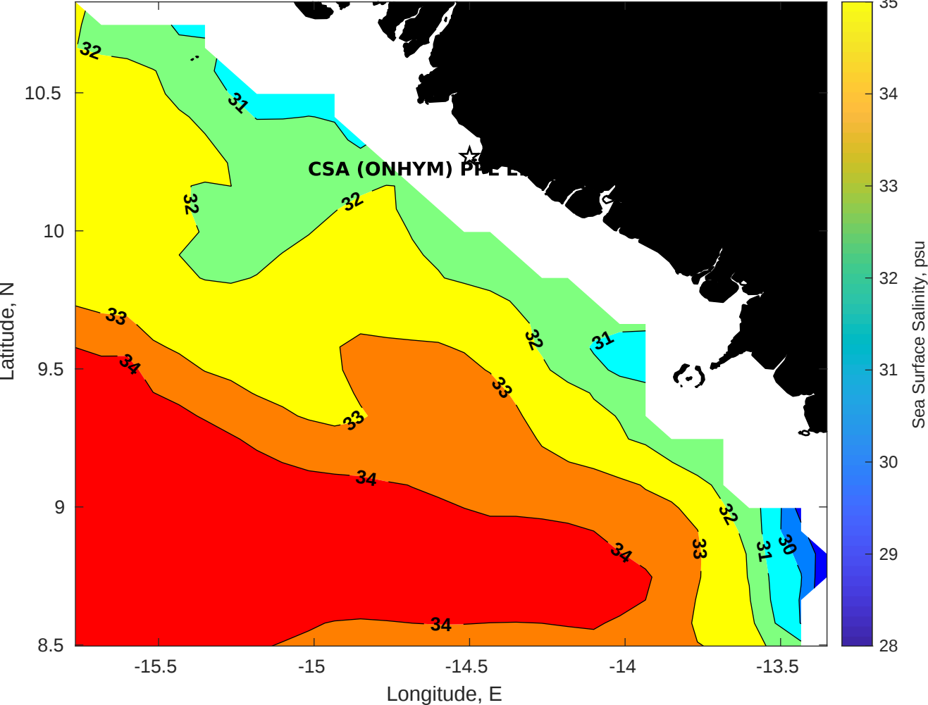
Surface Salinity for CSA (ONHYM) PPL EBS - Guinea at 18-Oct-2025 00:00:00
