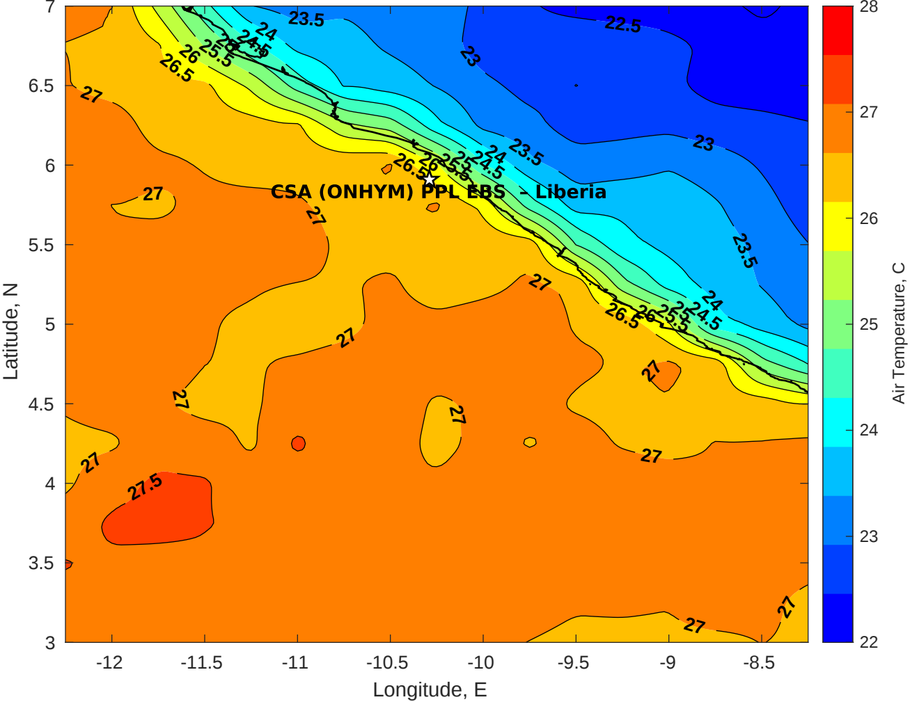
Air Temperature (C) for CSA (ONHYM) PPL EBS - Liberia at 19-Oct-2025
