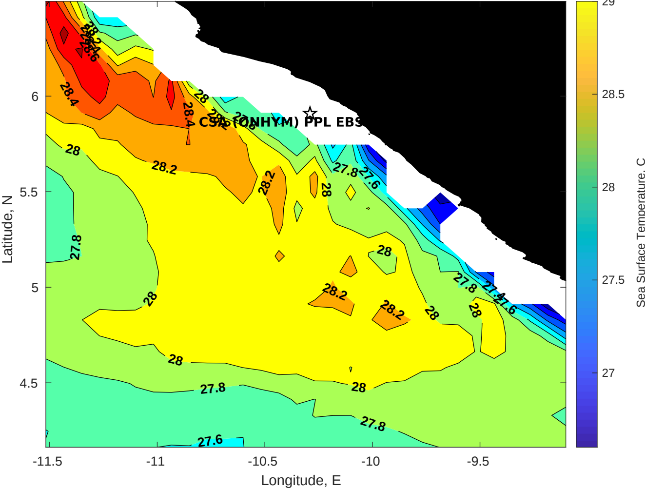
SST for CSA (ONHYM) PPL EBS - Liberia at 18-Oct-2025 00:00:00
