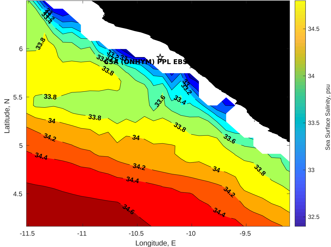
Surface Salinity for CSA (ONHYM) PPL EBS - Liberia at 18-Oct-2025 00:00:00
